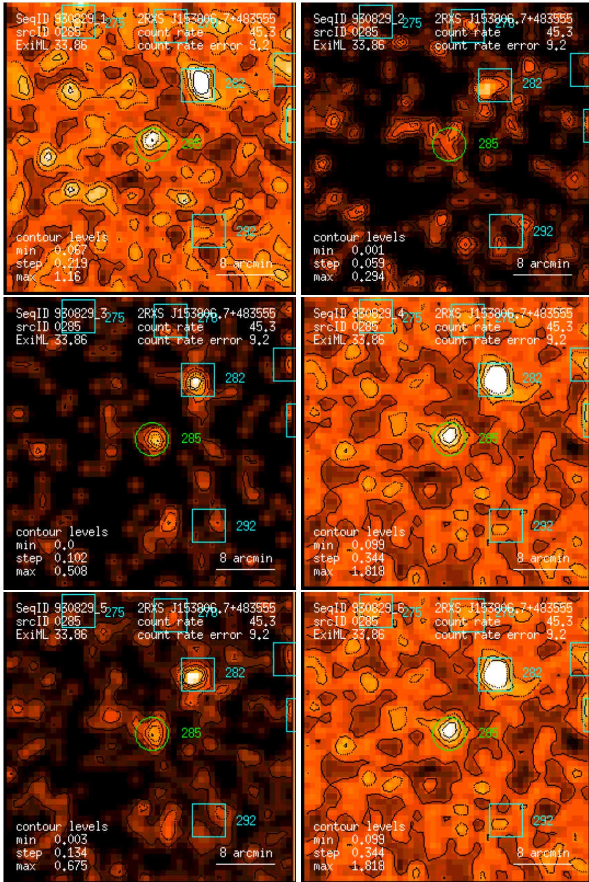
Figure 285: RASS 930829: detection 0285: band rate images, Gaussian filter: (1) PSPC channels 11 – 41, (2) 52 – 90, (3) 91 – 201, (4) 11 – 235, (5) 52 – 201, (6) 11 – 201. Broad band rates in counts/ks. Band rate contour levels in counts/ks/arcmin 2 .
