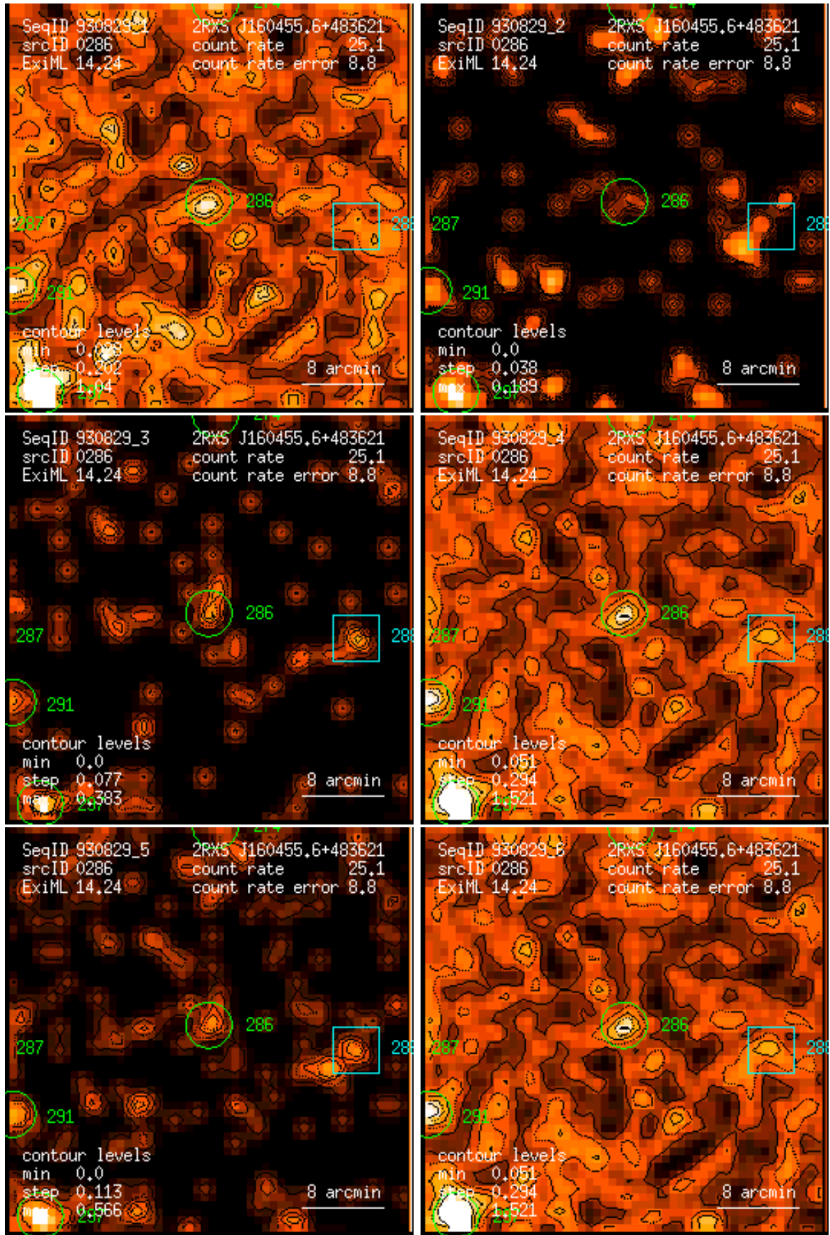
Figure 286: RASS 930829: detection 0286: band rate images, Gaussian filter: (1) PSPC channels 11 – 41, (2) 52 – 90, (3) 91 – 201, (4) 11 – 235, (5) 52 – 201, (6) 11 – 201. Broad band rates in counts/ks. Band rate contour levels in counts/ks/arcmin 2 .
