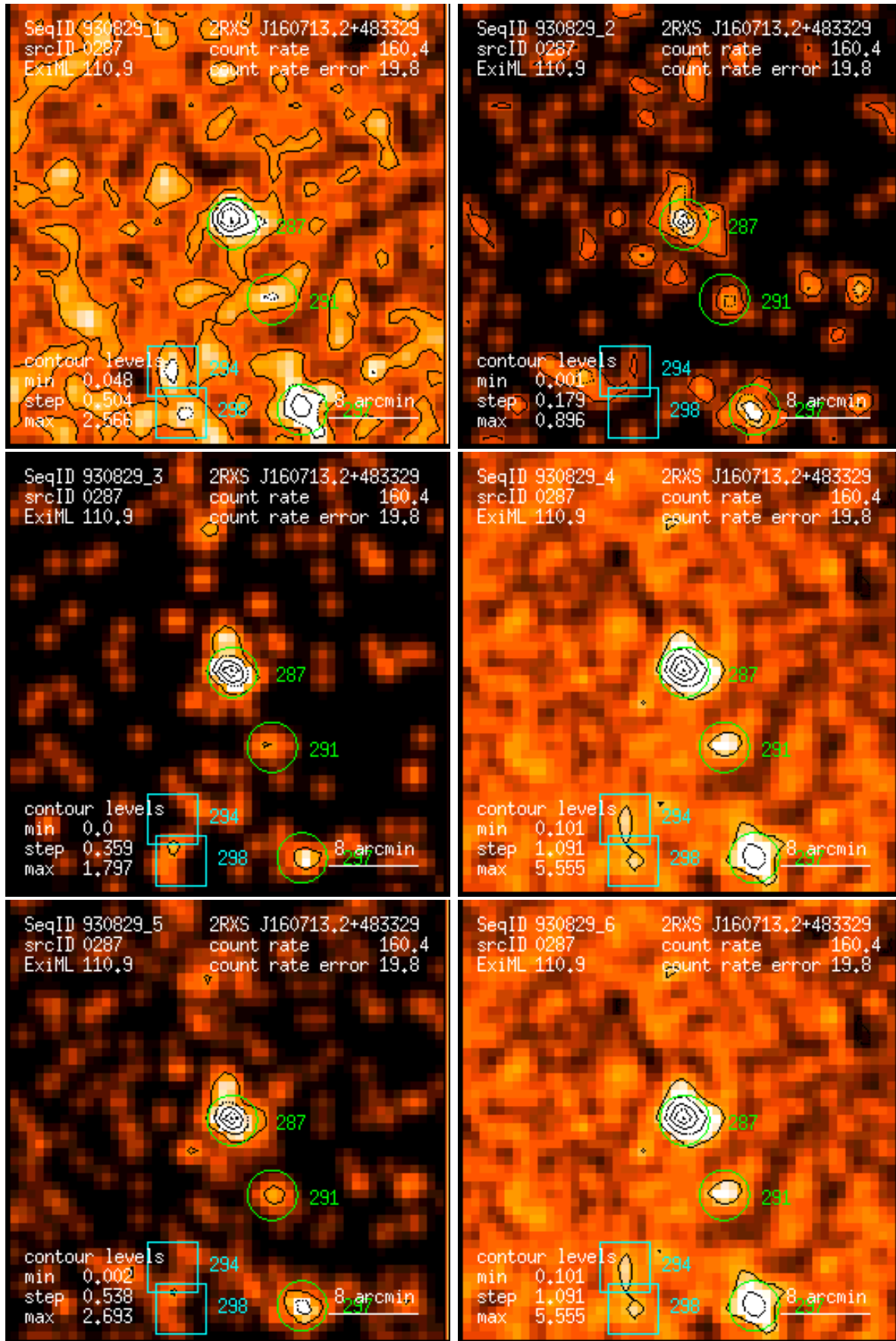
Figure 287: RASS 930829: detection 0287: band rate images, Gaussian filter: (1) PSPC channels 11 – 41, (2) 52 – 90, (3) 91 – 201, (4) 11 – 235, (5) 52 – 201, (6) 11 – 201. Broad band rates in counts/ks. Band rate contour levels in counts/ks/arcmin 2 .
