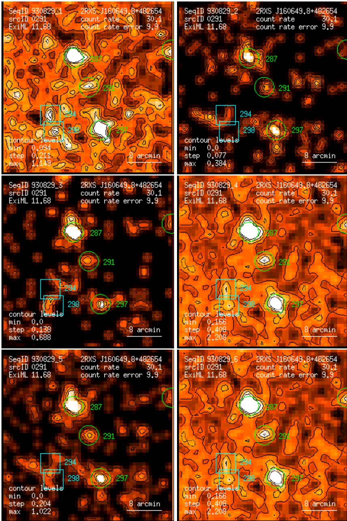
Figure 291: RASS 930829: detection 0291: band rate images, Gaussian filter: (1) PSPC channels 11 – 41, (2) 52 – 90, (3) 91 – 201, (4) 11 – 235, (5) 52 – 201, (6) 11 – 201. Broad band rates in counts/ks. Band rate contour levels in counts/ks/arcmin 2 .
