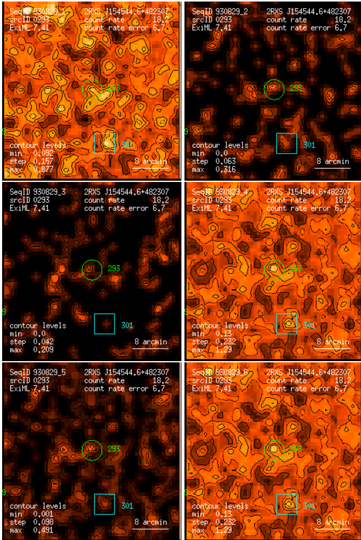
Figure 293: RASS 930829: detection 0293: band rate images, Gaussian filter: (1) PSPC channels 11 – 41, (2) 52 – 90, (3) 91 – 201, (4) 11 – 235, (5) 52 – 201, (6) 11 – 201. Broad band rates in counts/ks. Band rate contour levels in counts/ks/arcmin 2 .
