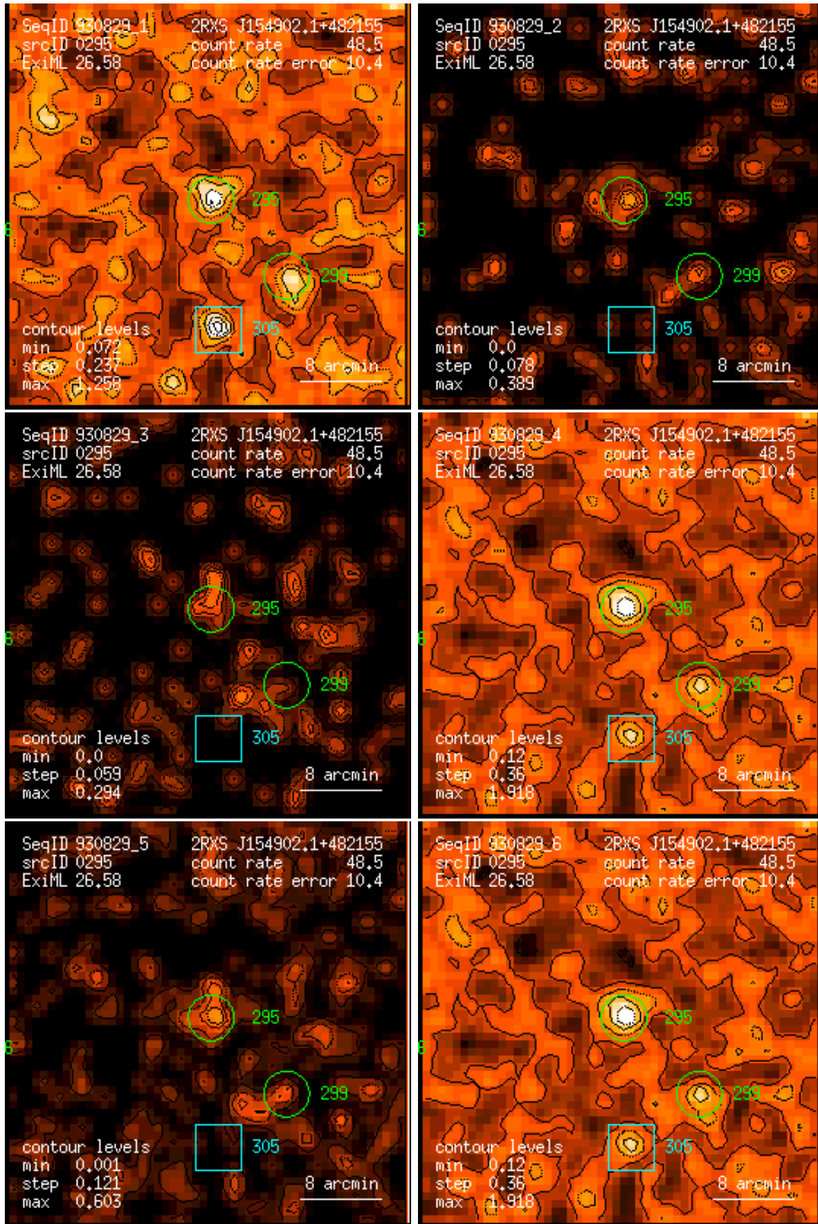
Figure 295: RASS 930829: detection 0295: band rate images, Gaussian filter: (1) PSPC channels 11 – 41, (2) 52 – 90, (3) 91 – 201, (4) 11 – 235, (5) 52 – 201, (6) 11 – 201. Broad band rates in counts/ks. Band rate contour levels in counts/ks/arcmin 2 .
