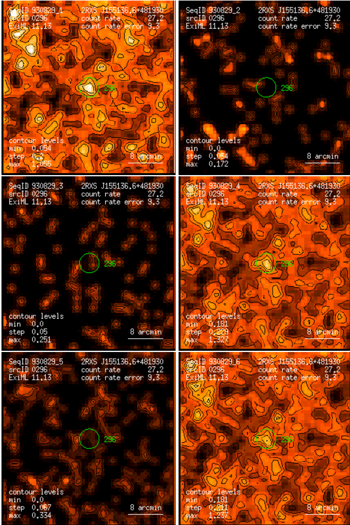
Figure 296: RASS 930829: detection 0296: band rate images, Gaussian filter: (1) PSPC channels 11 – 41, (2) 52 – 90, (3) 91 – 201, (4) 11 – 235, (5) 52 – 201, (6) 11 – 201. Broad band rates in counts/ks. Band rate contour levels in counts/ks/arcmin 2 .
