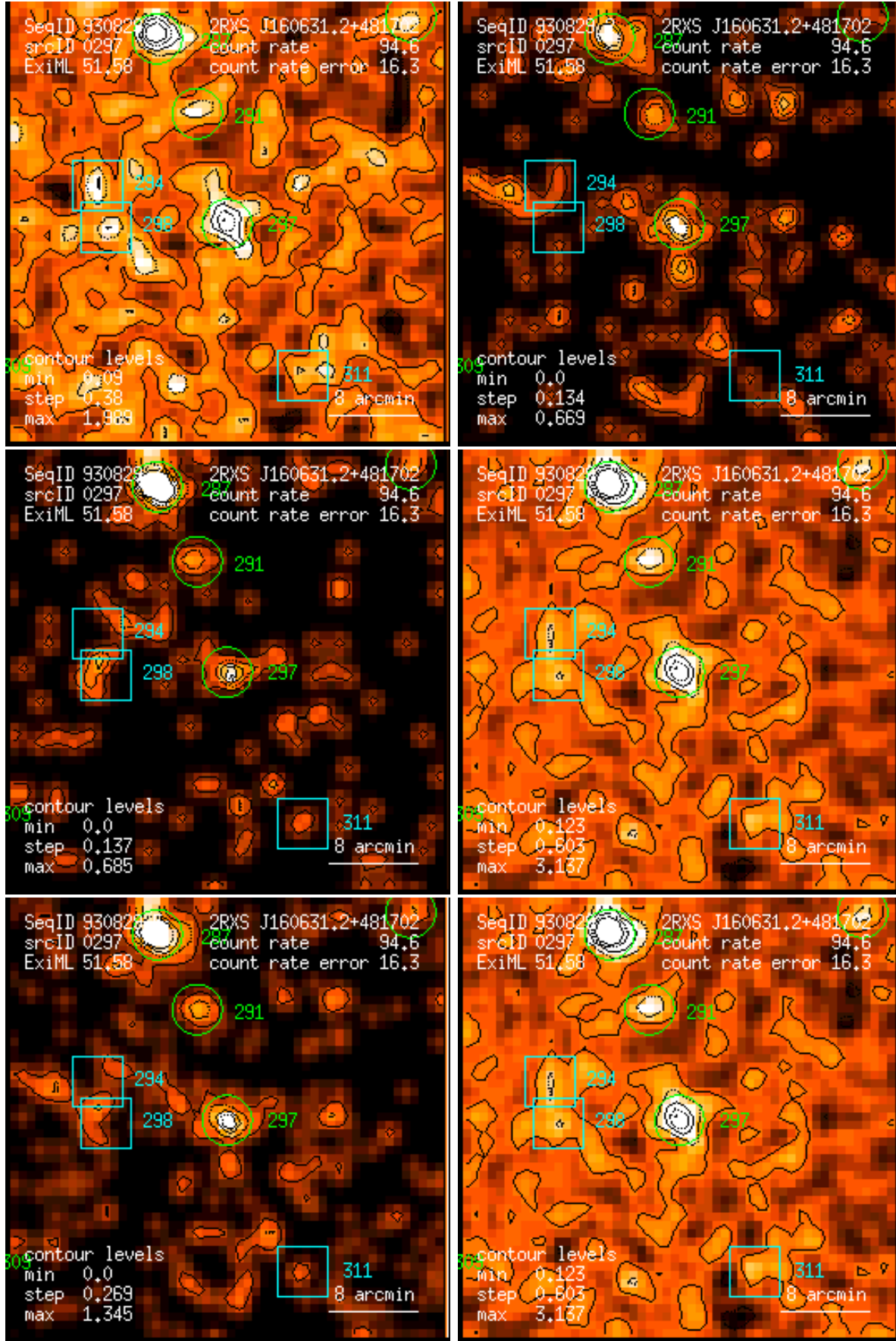
Figure 297: RASS 930829: detection 0297: band rate images, Gaussian filter: (1) PSPC channels 11 – 41, (2) 52 – 90, (3) 91 – 201, (4) 11 – 235, (5) 52 – 201, (6) 11 – 201. Broad band rates in counts/ks. Band rate contour levels in counts/ks/arcmin 2 .
