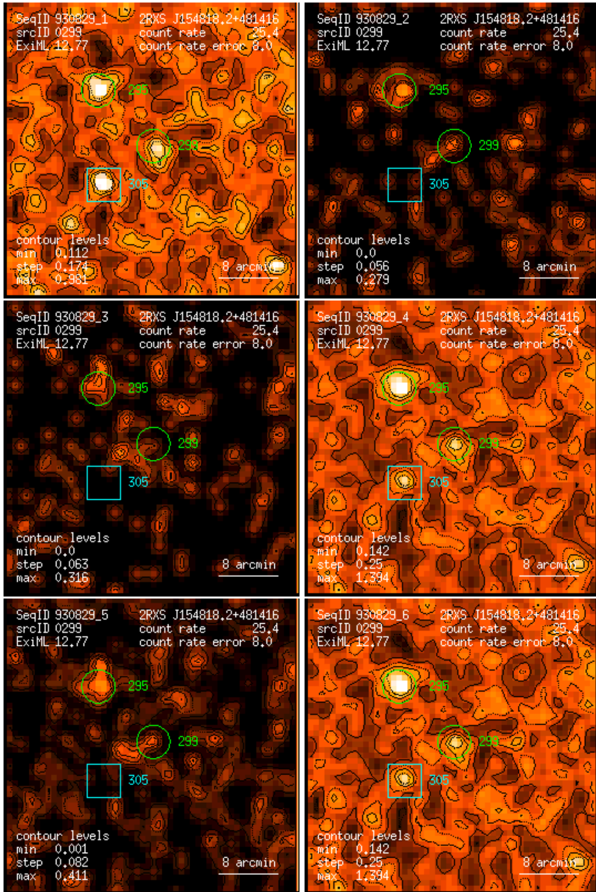
Figure 299: RASS 930829: detection 0299: band rate images, Gaussian filter: (1) PSPC channels 11 – 41, (2) 52 – 90, (3) 91 – 201, (4) 11 – 235, (5) 52 – 201, (6) 11 – 201. Broad band rates in counts/ks. Band rate contour levels in counts/ks/arcmin 2 .
