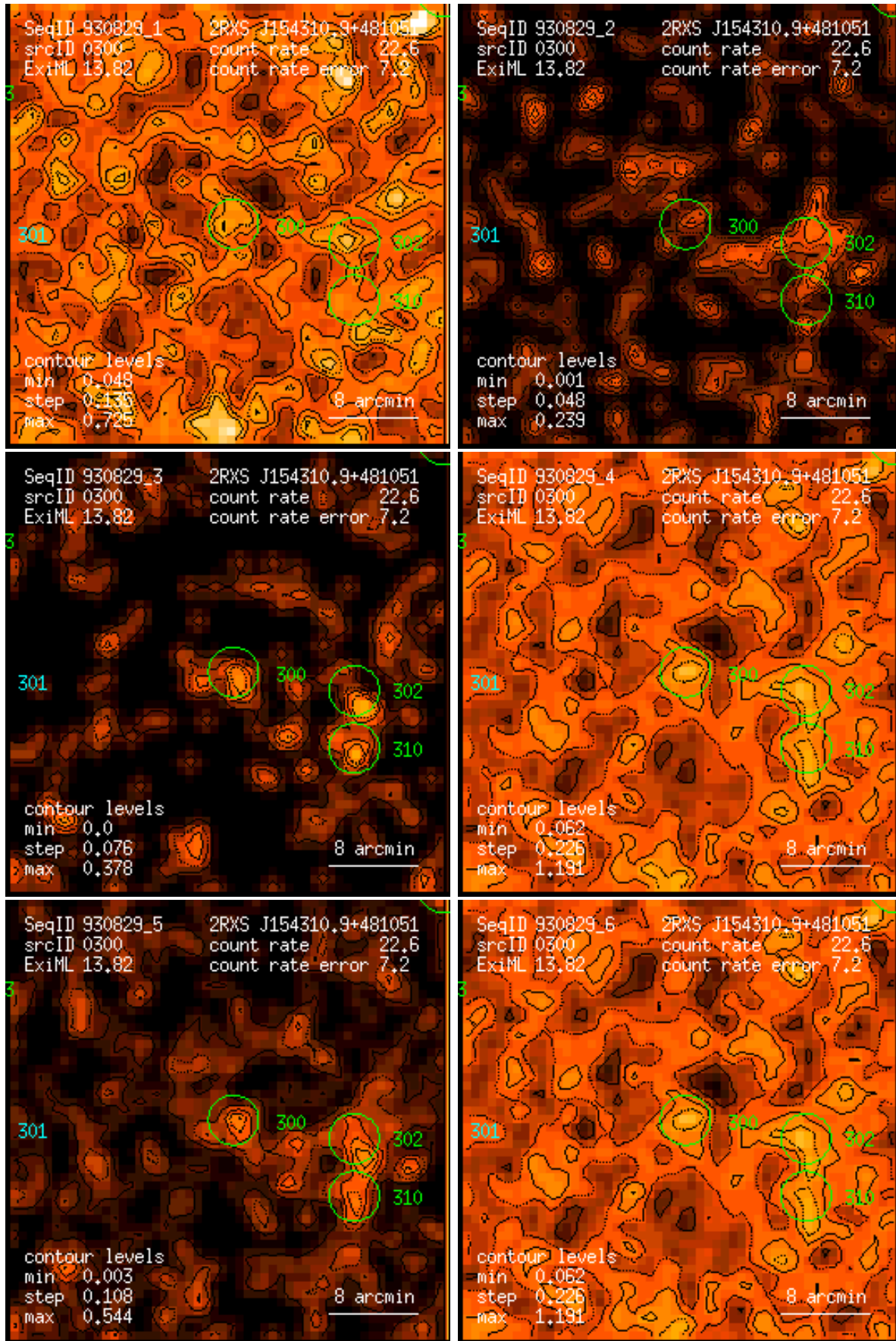
Figure 300: RASS 930829: detection 0300: band rate images, Gaussian filter: (1) PSPC channels 11 – 41, (2) 52 – 90, (3) 91 – 201, (4) 11 – 235, (5) 52 – 201, (6) 11 – 201. Broad band rates in counts/ks. Band rate contour levels in counts/ks/arcmin 2 .
