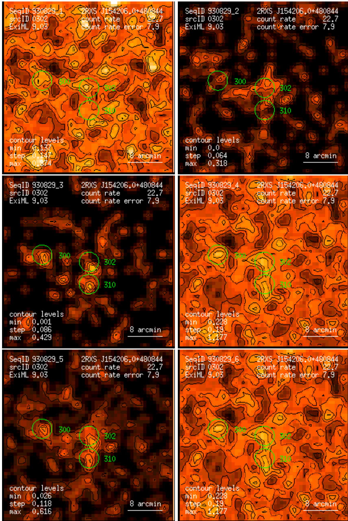
Figure 302: RASS 930829: detection 0302: band rate images, Gaussian filter: (1) PSPC channels 11 – 41, (2) 52 – 90, (3) 91 – 201, (4) 11 – 235, (5) 52 – 201, (6) 11 – 201. Broad band rates in counts/ks. Band rate contour levels in counts/ks/arcmin 2 .
