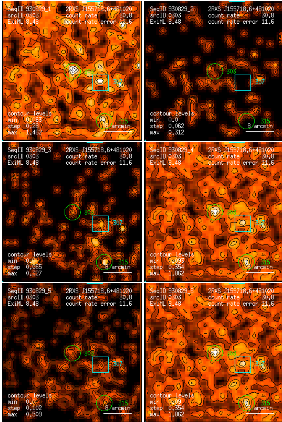
Figure 303: RASS 930829: detection 0303: band rate images, Gaussian filter: (1) PSPC channels 11 – 41, (2) 52 – 90, (3) 91 – 201, (4) 11 – 235, (5) 52 – 201, (6) 11 – 201. Broad band rates in counts/ks. Band rate contour levels in counts/ks/arcmin 2 .
