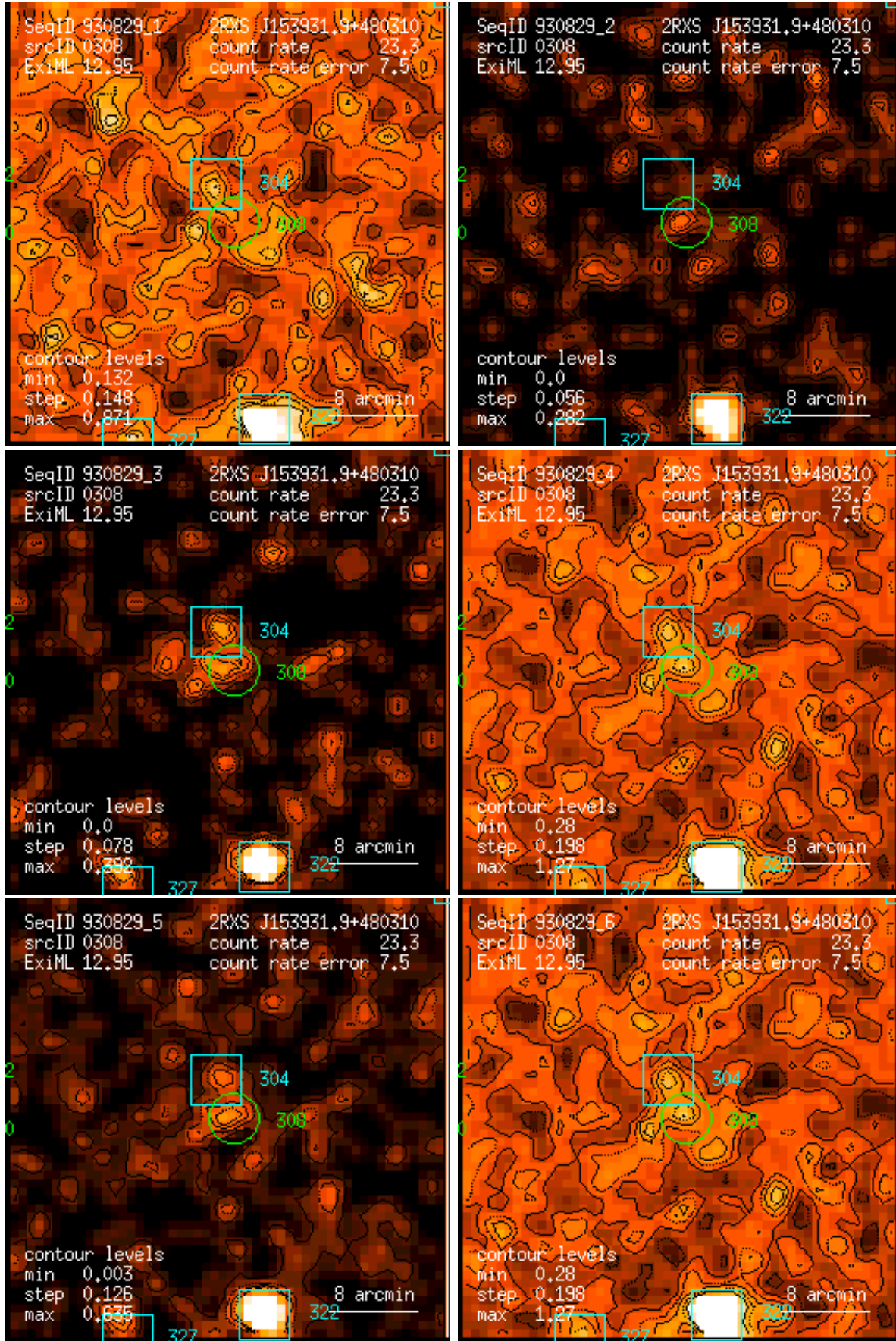
Figure 308: RASS 930829: detection 0308: band rate images, Gaussian filter: (1) PSPC channels 11 – 41, (2) 52 – 90, (3) 91 – 201, (4) 11 – 235, (5) 52 – 201, (6) 11 – 201. Broad band rates in counts/ks. Band rate contour levels in counts/ks/arcmin 2 .
