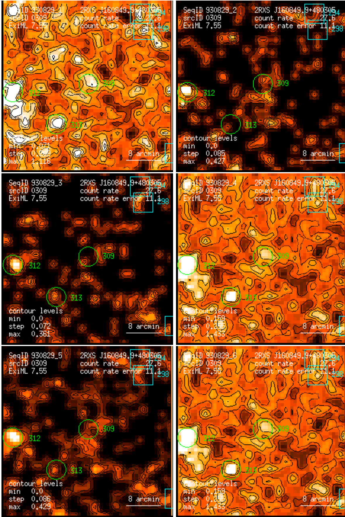
Figure 309: RASS 930829: detection 0309: band rate images, Gaussian filter: (1) PSPC channels 11 – 41, (2) 52 – 90, (3) 91 – 201, (4) 11 – 235, (5) 52 – 201, (6) 11 – 201. Broad band rates in counts/ks. Band rate contour levels in counts/ks/arcmin 2 .
