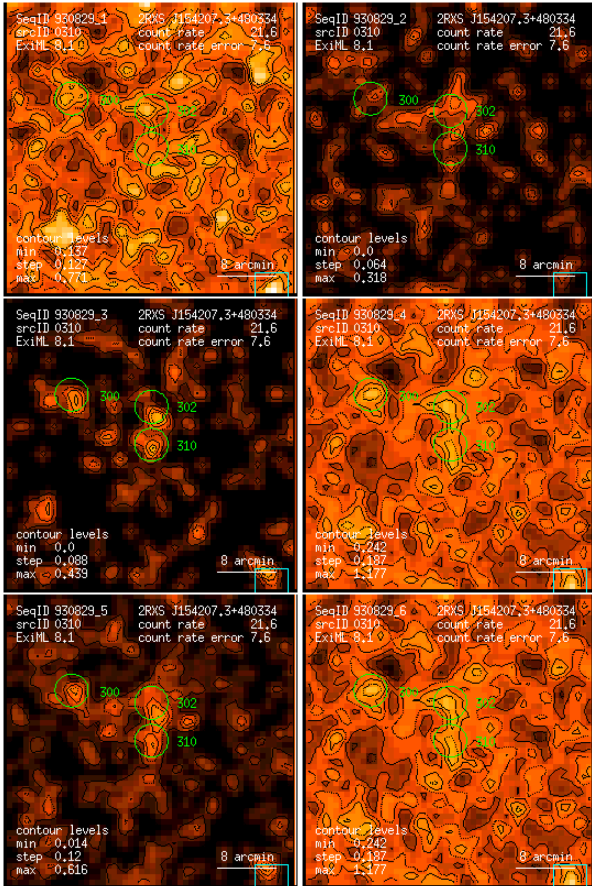
Figure 310: RASS 930829: detection 0310: band rate images, Gaussian filter: (1) PSPC channels 11 – 41, (2) 52 – 90, (3) 91 – 201, (4) 11 – 235, (5) 52 – 201, (6) 11 – 201. Broad band rates in counts/ks. Band rate contour levels in counts/ks/arcmin 2 .
