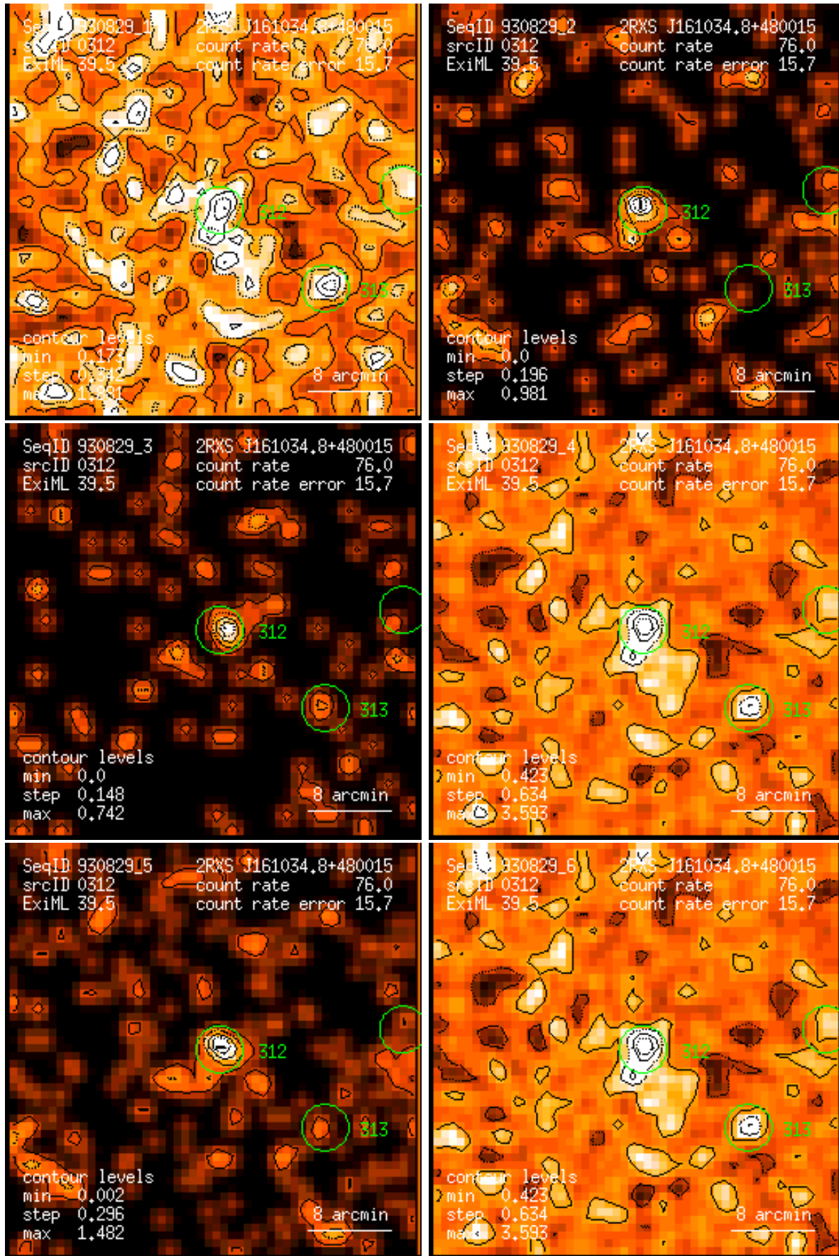
Figure 312: RASS 930829: detection 0312: band rate images, Gaussian filter: (1) PSPC channels 11 – 41, (2) 52 – 90, (3) 91 – 201, (4) 11 – 235, (5) 52 – 201, (6) 11 – 201. Broad band rates in counts/ks. Band rate contour levels in counts/ks/arcmin 2 .
