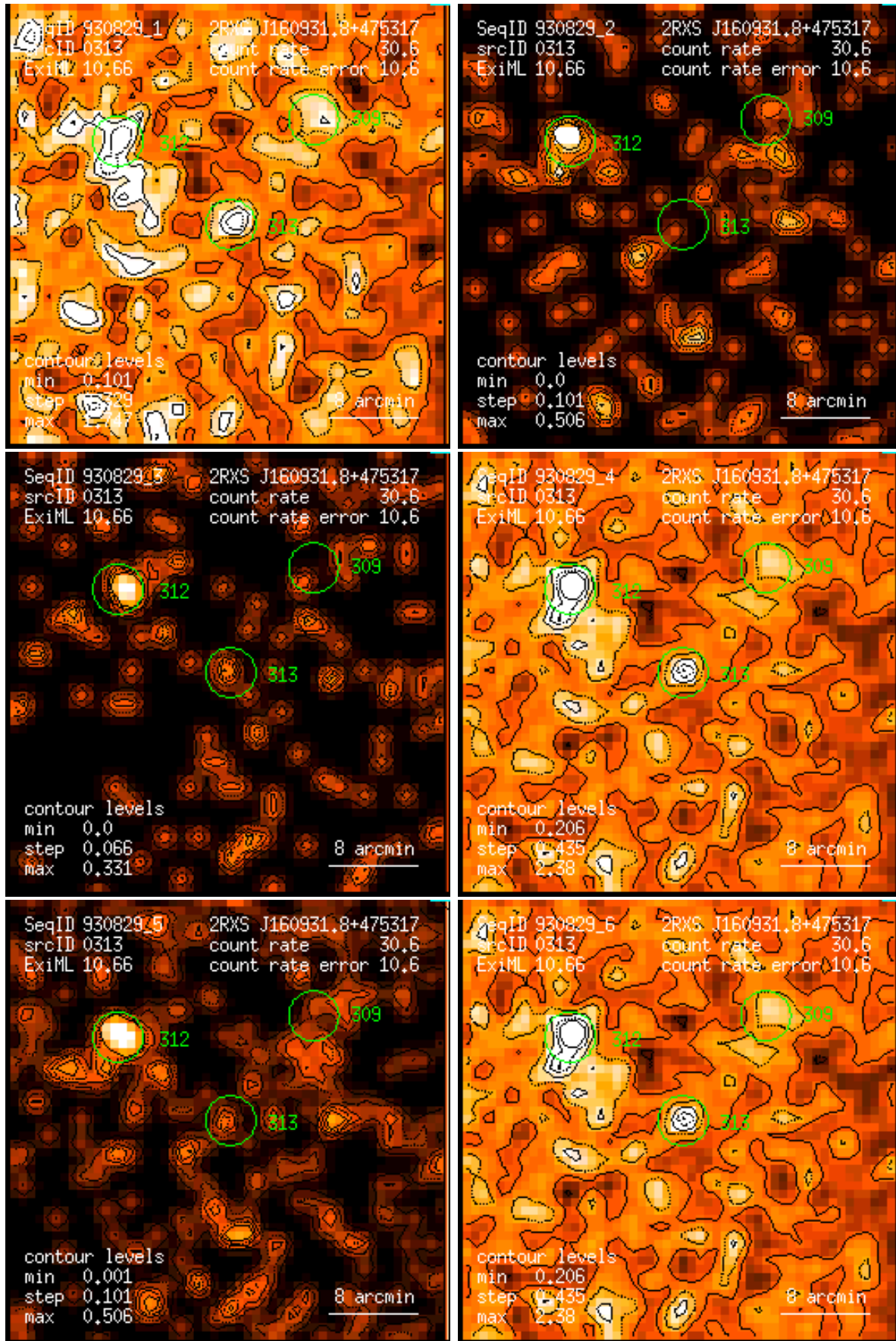
Figure 313: RASS 930829: detection 0313: band rate images, Gaussian filter: (1) PSPC channels 11 – 41, (2) 52 – 90, (3) 91 – 201, (4) 11 – 235, (5) 52 – 201, (6) 11 – 201. Broad band rates in counts/ks. Band rate contour levels in counts/ks/arcmin 2 .
