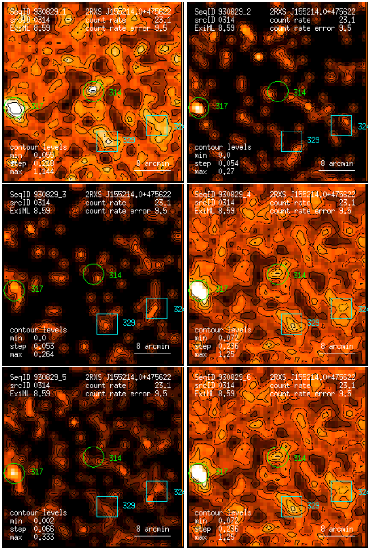
Figure 314: RASS 930829: detection 0314: band rate images, Gaussian filter: (1) PSPC channels 11 – 41, (2) 52 – 90, (3) 91 – 201, (4) 11 – 235, (5) 52 – 201, (6) 11 – 201. Broad band rates in counts/ks. Band rate contour levels in counts/ks/arcmin 2 .
