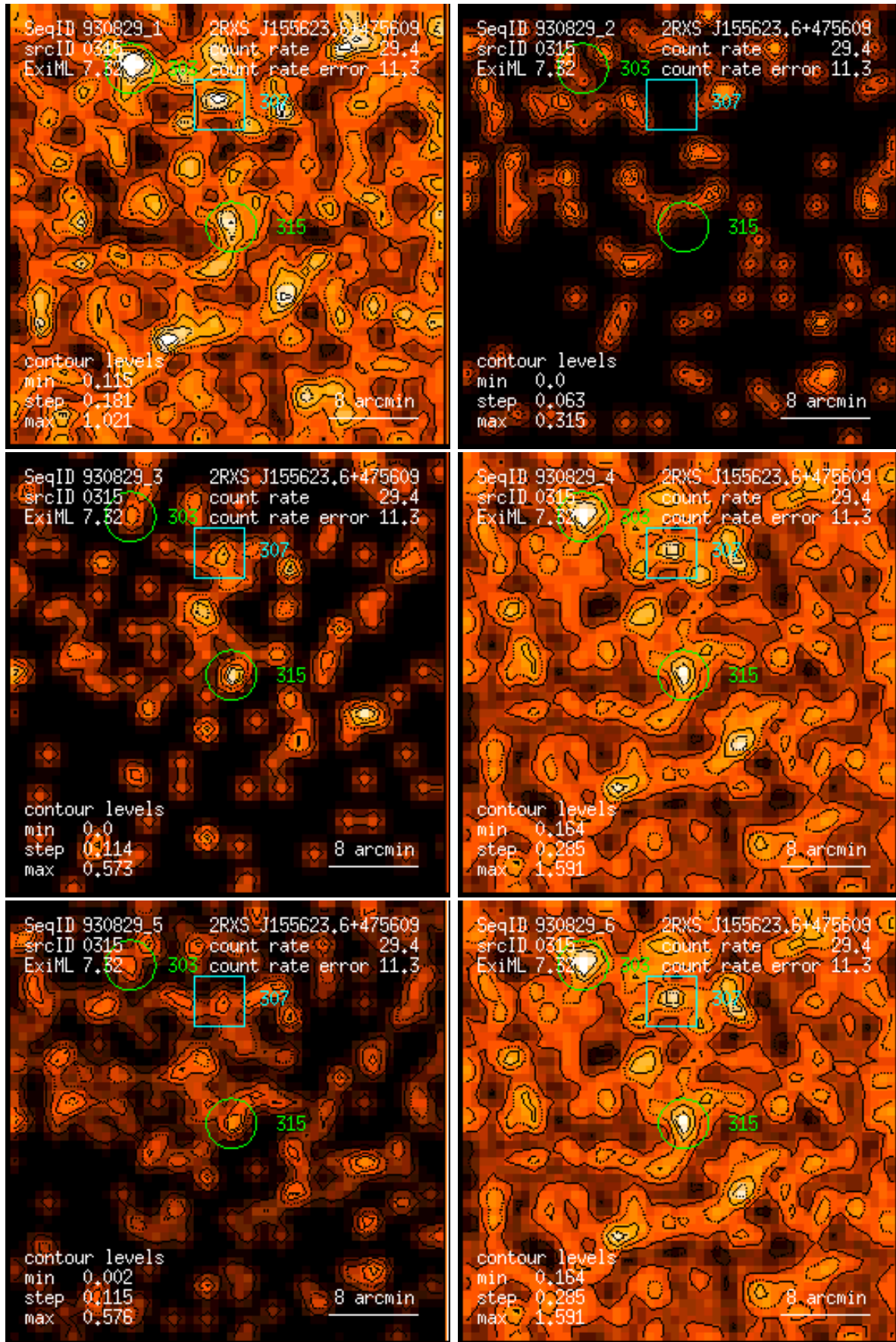
Figure 315: RASS 930829: detection 0315: band rate images, Gaussian filter: (1) PSPC channels 11 – 41, (2) 52 – 90, (3) 91 – 201, (4) 11 – 235, (5) 52 – 201, (6) 11 – 201. Broad band rates in counts/ks. Band rate contour levels in counts/ks/arcmin 2 .
