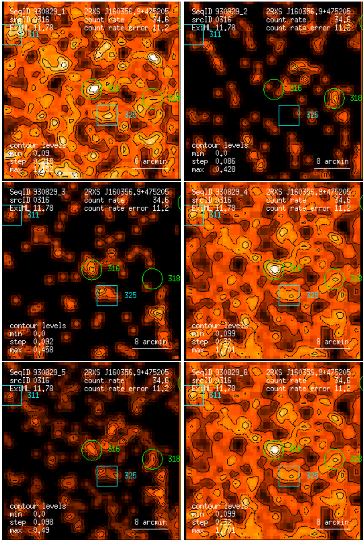
Figure 316: RASS 930829: detection 0316: band rate images, Gaussian filter: (1) PSPC channels 11 – 41, (2) 52 – 90, (3) 91 – 201, (4) 11 – 235, (5) 52 – 201, (6) 11 – 201. Broad band rates in counts/ks. Band rate contour levels in counts/ks/arcmin 2 .
