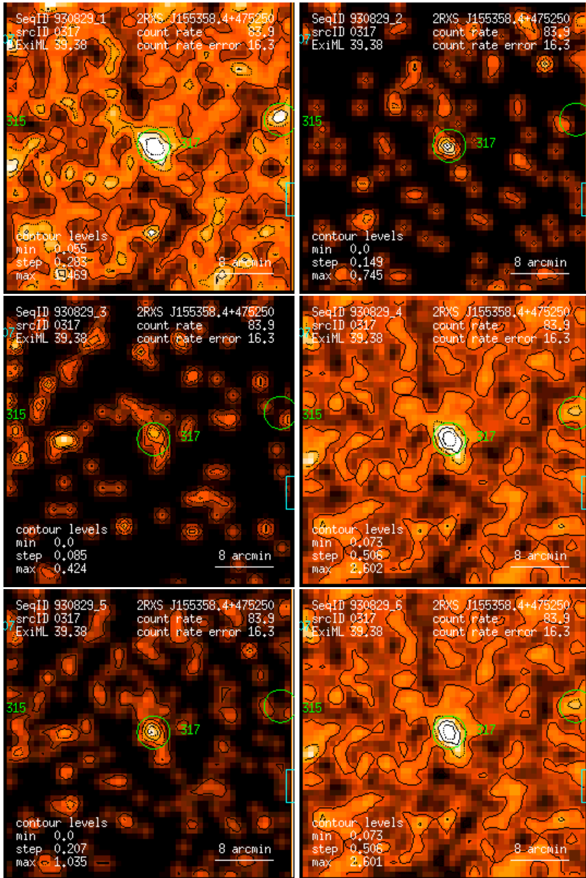
Figure 317: RASS 930829: detection 0317: band rate images, Gaussian filter: (1) PSPC channels 11 – 41, (2) 52 – 90, (3) 91 – 201, (4) 11 – 235, (5) 52 – 201, (6) 11 – 201. Broad band rates in counts/ks. Band rate contour levels in counts/ks/arcmin 2 .
