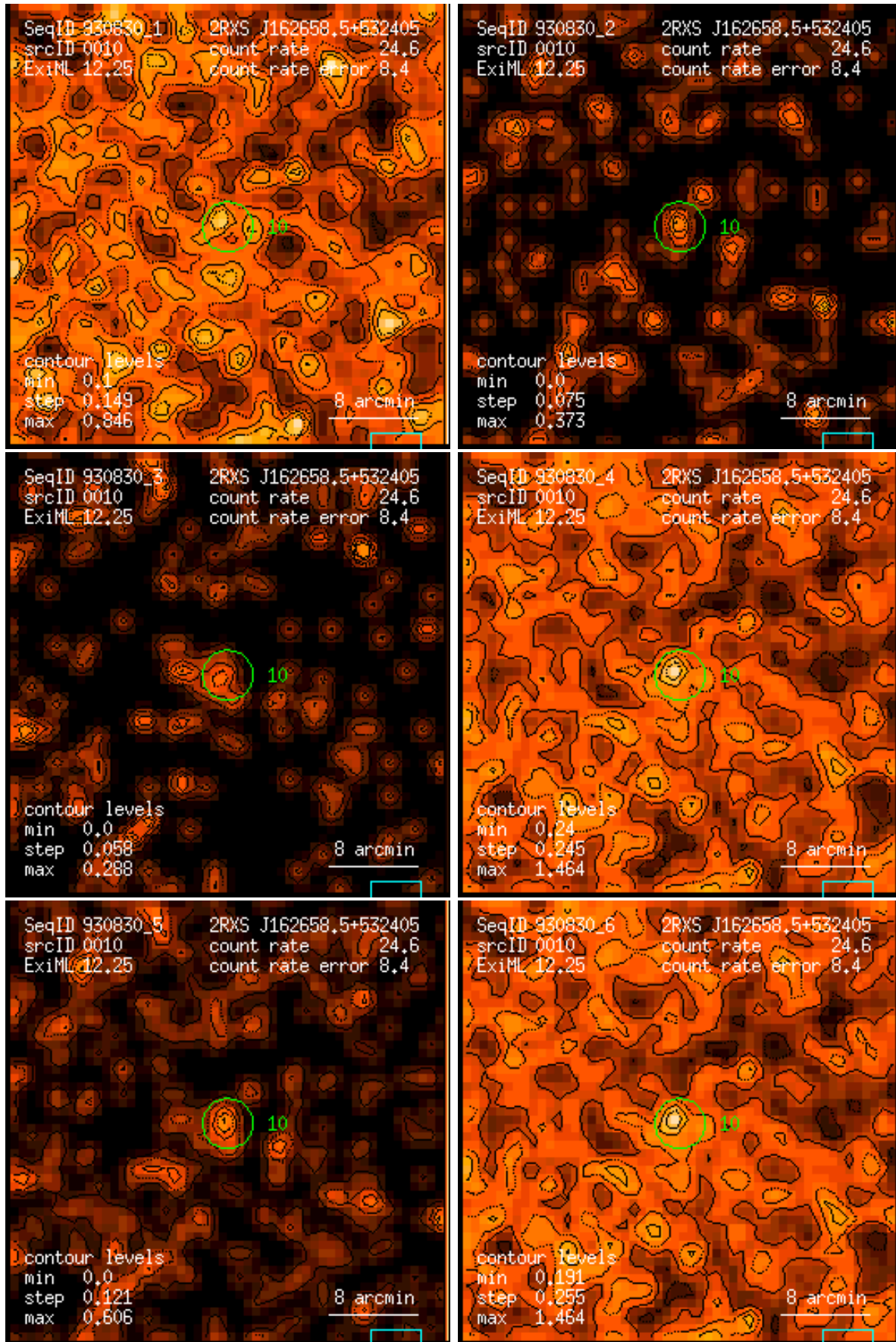
Figure 10: RASS 930830: detection 0010: band rate images, Gaussian filter: (1) PSPC channels 11 – 41, (2) 52 – 90, (3) 91 – 201, (4) 11 – 235, (5) 52 – 201, (6) 11 – 201. Broad band rates in counts/ks. Band rate contour levels in counts/ks/arcmin 2 .
