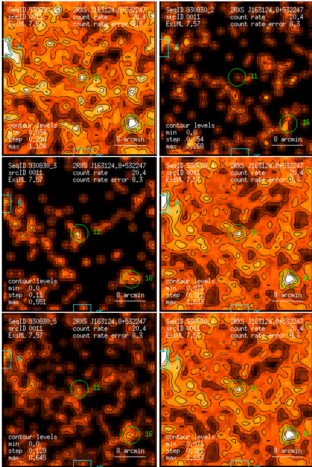
Figure 11: RASS 930830: detection 0011: band rate images, Gaussian filter: (1) PSPC channels 11 – 41, (2) 52 – 90, (3) 91 – 201, (4) 11 – 235, (5) 52 – 201, (6) 11 – 201. Broad band rates in counts/ks. Band rate contour levels in counts/ks/arcmin 2 .
