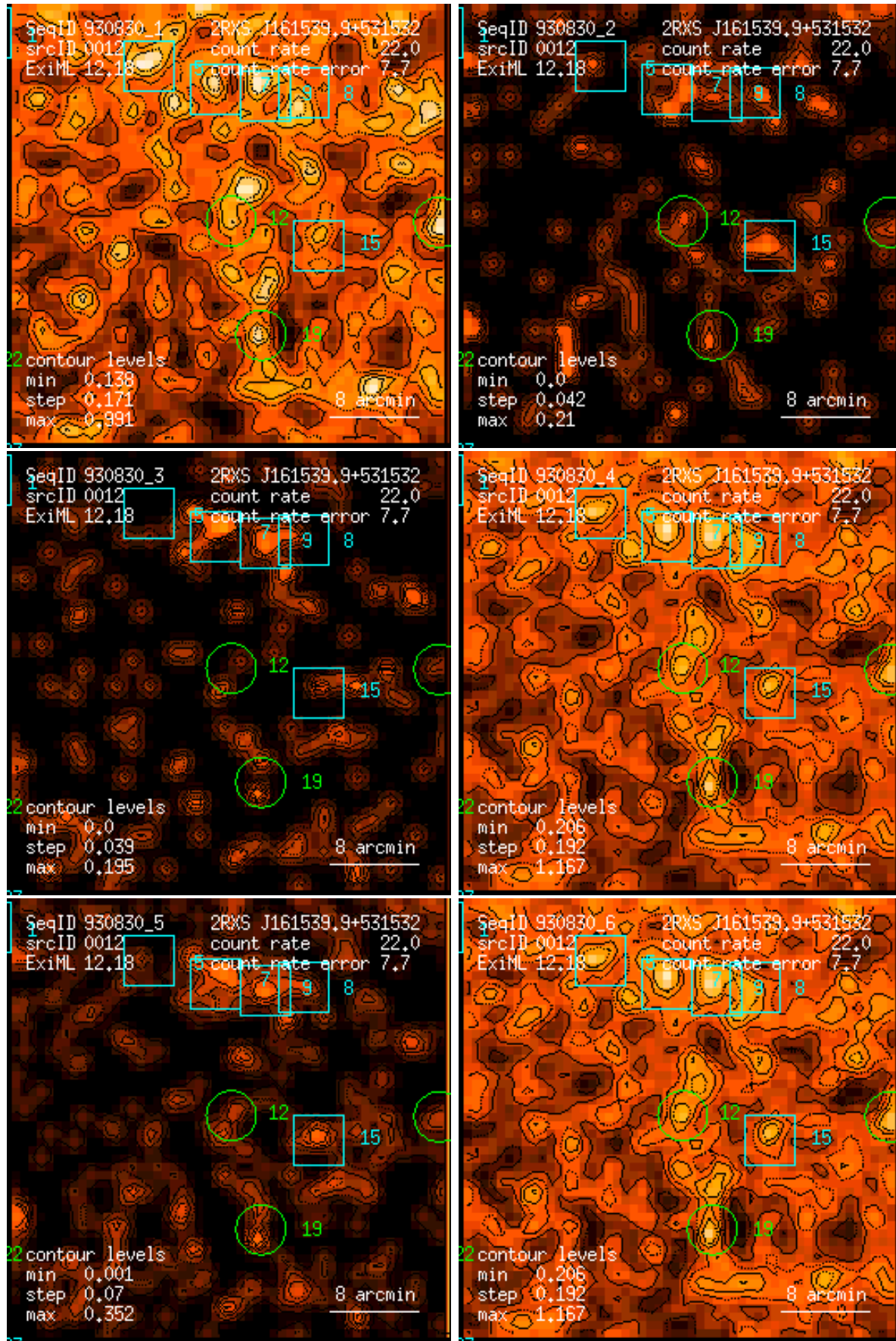
Figure 12: RASS 930830: detection 0012: band rate images, Gaussian filter: (1) PSPC channels 11 – 41, (2) 52 – 90, (3) 91 – 201, (4) 11 – 235, (5) 52 – 201, (6) 11 – 201. Broad band rates in counts/ks. Band rate contour levels in counts/ks/arcmin 2 .
