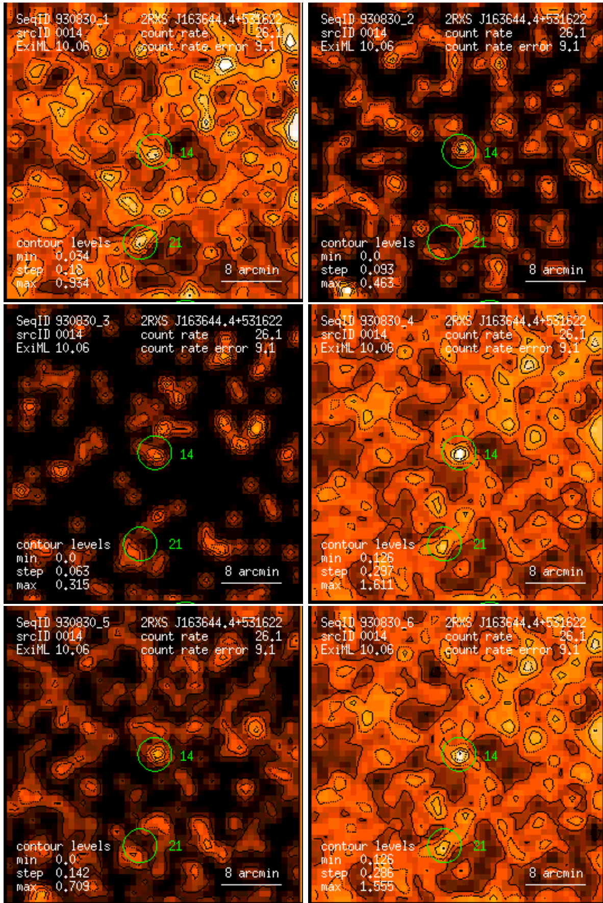
Figure 14: RASS 930830: detection 0014: band rate images, Gaussian filter: (1) PSPC channels 11 – 41, (2) 52 – 90, (3) 91 – 201, (4) 11 – 235, (5) 52 – 201, (6) 11 – 201. Broad band rates in counts/ks. Band rate contour levels in counts/ks/arcmin 2 .
