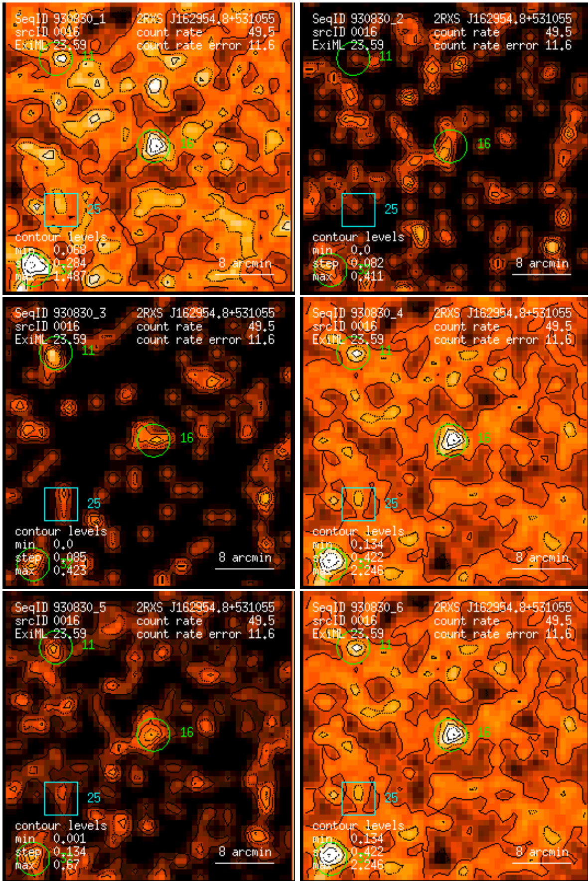
Figure 16: RASS 930830: detection 0016: band rate images, Gaussian filter: (1) PSPC channels 11 – 41, (2) 52 – 90, (3) 91 – 201, (4) 11 – 235, (5) 52 – 201, (6) 11 – 201. Broad band rates in counts/ks. Band rate contour levels in counts/ks/arcmin 2 .
