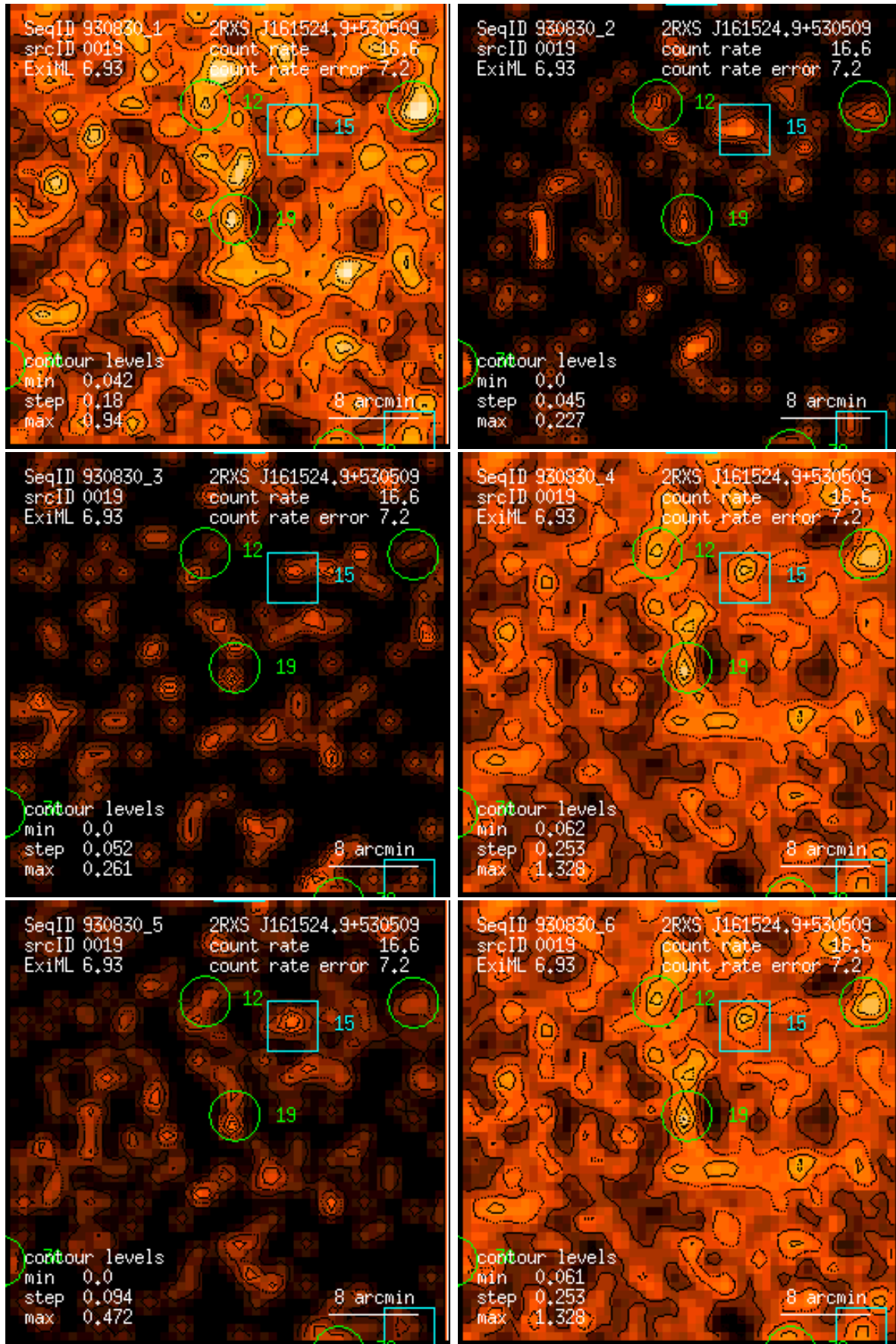
Figure 19: RASS 930830: detection 0019: band rate images, Gaussian filter: (1) PSPC channels 11 – 41, (2) 52 – 90, (3) 91 – 201, (4) 11 – 235, (5) 52 – 201, (6) 11 – 201. Broad band rates in counts/ks. Band rate contour levels in counts/ks/arcmin 2 .
