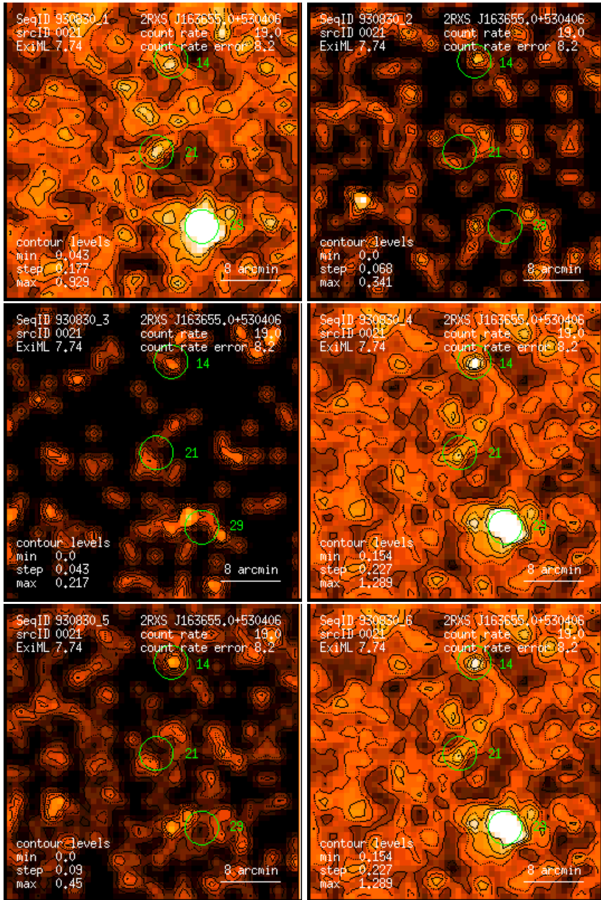
Figure 21: RASS 930830: detection 0021: band rate images, Gaussian filter: (1) PSPC channels 11 – 41, (2) 52 – 90, (3) 91 – 201, (4) 11 – 235, (5) 52 – 201, (6) 11 – 201. Broad band rates in counts/ks. Band rate contour levels in counts/ks/arcmin 2 .
