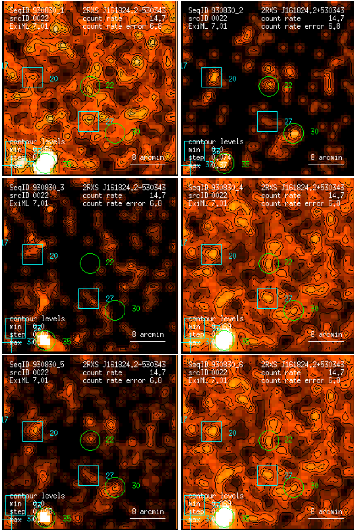
Figure 22: RASS 930830: detection 0022: band rate images, Gaussian filter: (1) PSPC channels 11 – 41, (2) 52 – 90, (3) 91 – 201, (4) 11 – 235, (5) 52 – 201, (6) 11 – 201. Broad band rates in counts/ks. Band rate contour levels in counts/ks/arcmin 2 .
