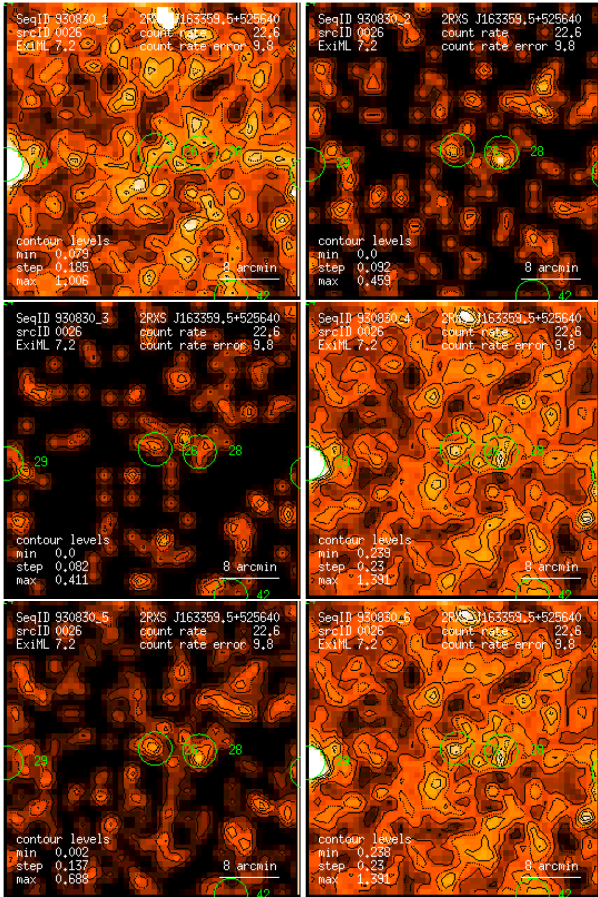
Figure 26: RASS 930830: detection 0026: band rate images, Gaussian filter: (1) PSPC channels 11 – 41, (2) 52 – 90, (3) 91 – 201, (4) 11 – 235, (5) 52 – 201, (6) 11 – 201. Broad band rates in counts/ks. Band rate contour levels in counts/ks/arcmin 2 .
