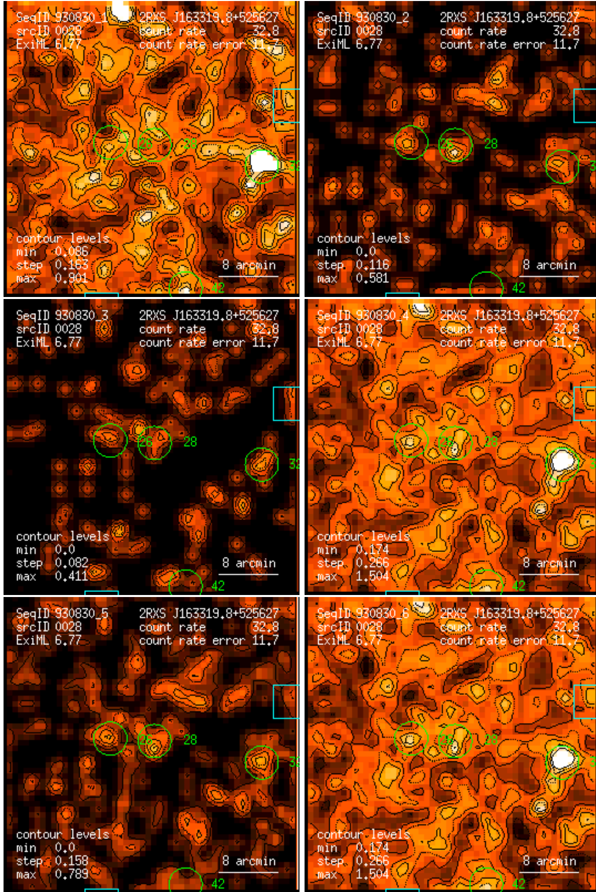
Figure 28: RASS 930830: detection 0028: band rate images, Gaussian filter: (1) PSPC channels 11 – 41, (2) 52 – 90, (3) 91 – 201, (4) 11 – 235, (5) 52 – 201, (6) 11 – 201. Broad band rates in counts/ks. Band rate contour levels in counts/ks/arcmin 2 .
