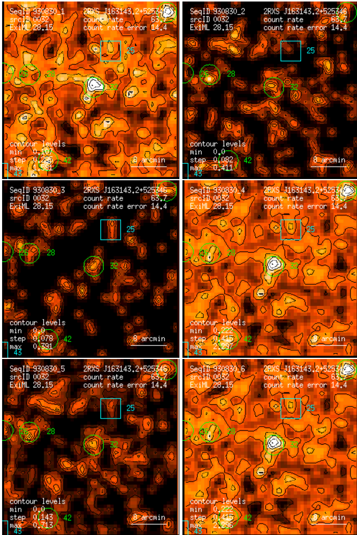
Figure 32: RASS 930830: detection 0032: band rate images, Gaussian filter: (1) PSPC channels 11 – 41, (2) 52 – 90, (3) 91 – 201, (4) 11 – 235, (5) 52 – 201, (6) 11 – 201. Broad band rates in counts/ks. Band rate contour levels in counts/ks/arcmin 2 .
