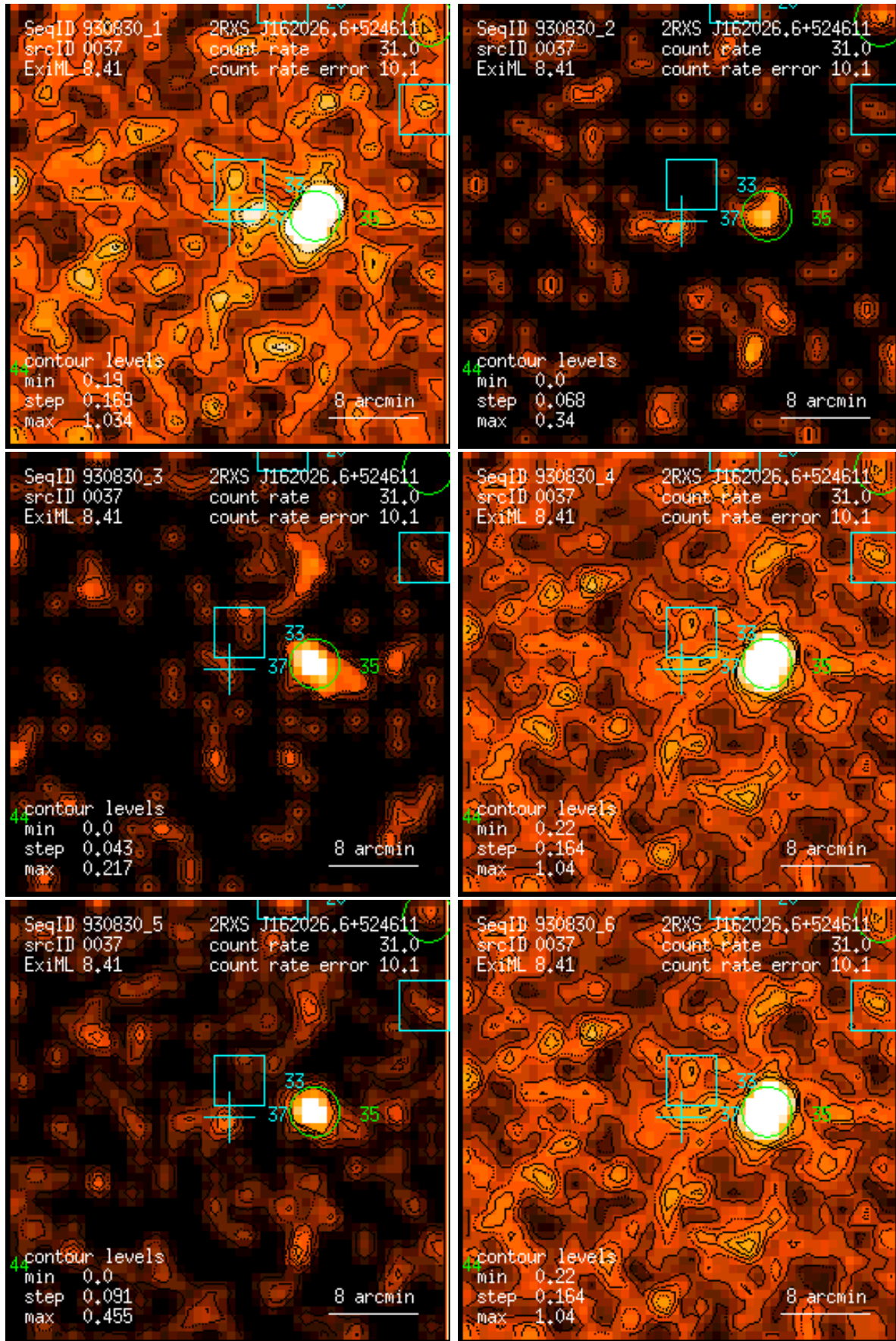
Figure 37: RASS 930830: detection 0037: band rate images, Gaussian filter: (1) PSPC channels 11 – 41, (2) 52 – 90, (3) 91 – 201, (4) 11 – 235, (5) 52 – 201, (6) 11 – 201. Broad band rates in counts/ks. Band rate contour levels in counts/ks/arcmin 2 .
