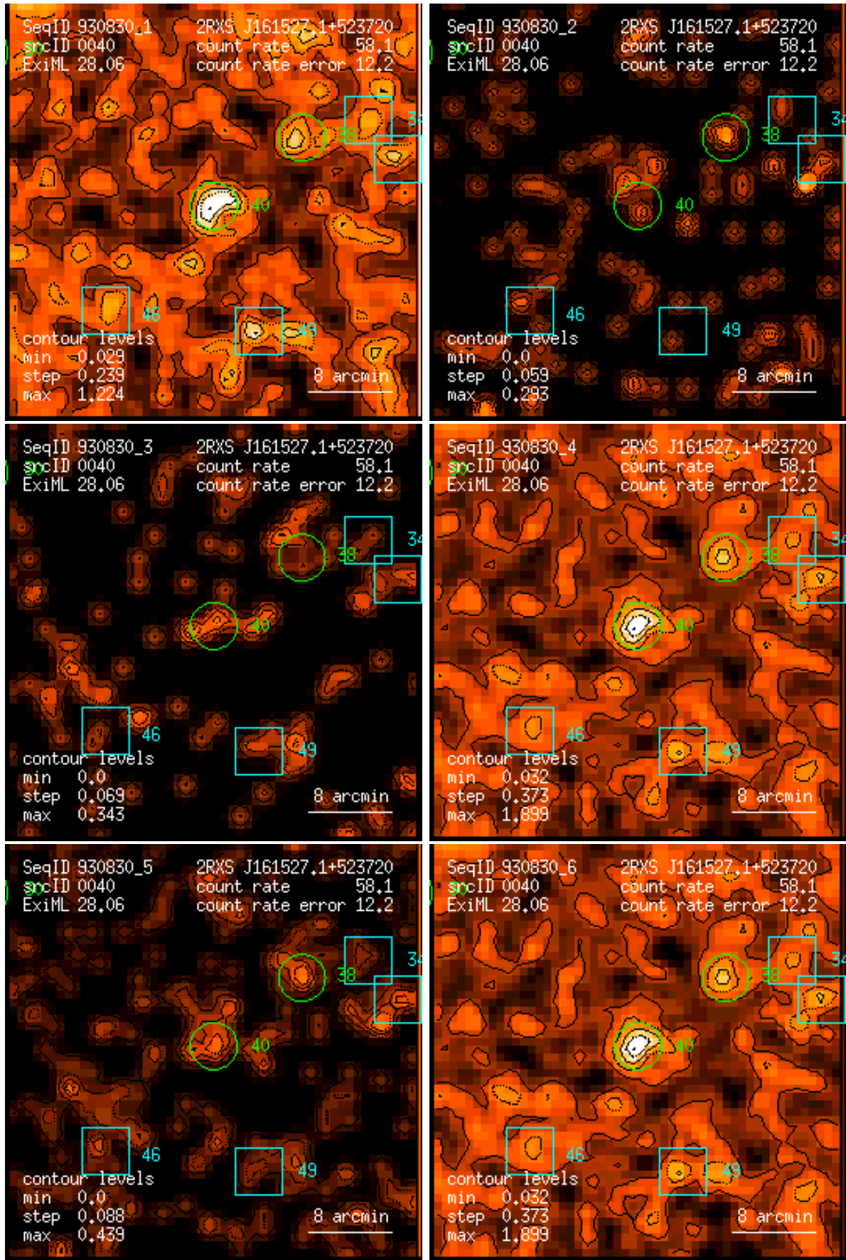
Figure 40: RASS 930830: detection 0040: band rate images, Gaussian filter: (1) PSPC channels 11 – 41, (2) 52 – 90, (3) 91 – 201, (4) 11 – 235, (5) 52 – 201, (6) 11 – 201. Broad band rates in counts/ks. Band rate contour levels in counts/ks/arcmin 2 .
