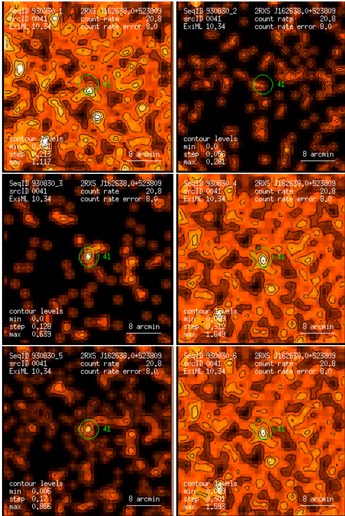
Figure 41: RASS 930830: detection 0041: band rate images, Gaussian filter: (1) PSPC channels 11 – 41, (2) 52 – 90, (3) 91 – 201, (4) 11 – 235, (5) 52 – 201, (6) 11 – 201. Broad band rates in counts/ks. Band rate contour levels in counts/ks/arcmin 2 .
