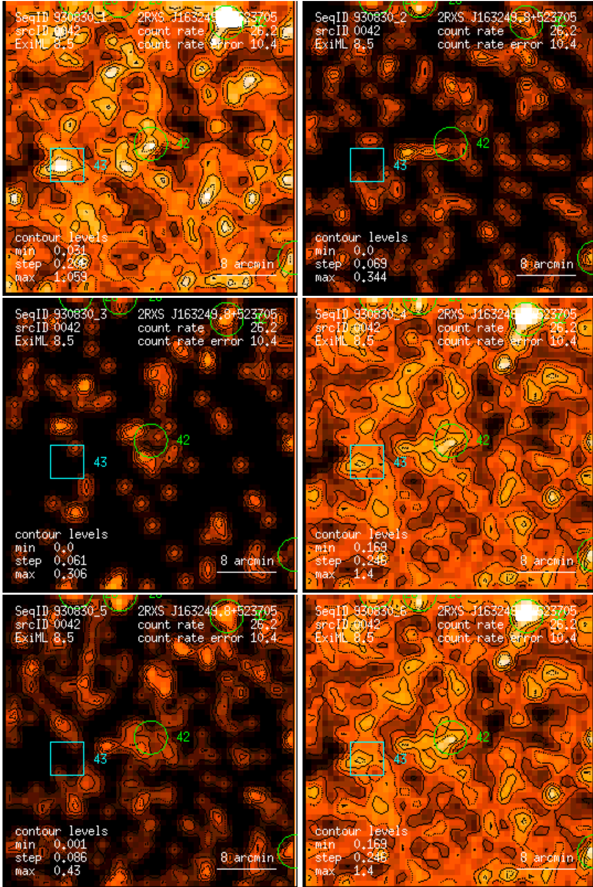
Figure 42: RASS 930830: detection 0042: band rate images, Gaussian filter: (1) PSPC channels 11 – 41, (2) 52 – 90, (3) 91 – 201, (4) 11 – 235, (5) 52 – 201, (6) 11 – 201. Broad band rates in counts/ks. Band rate contour levels in counts/ks/arcmin 2 .
