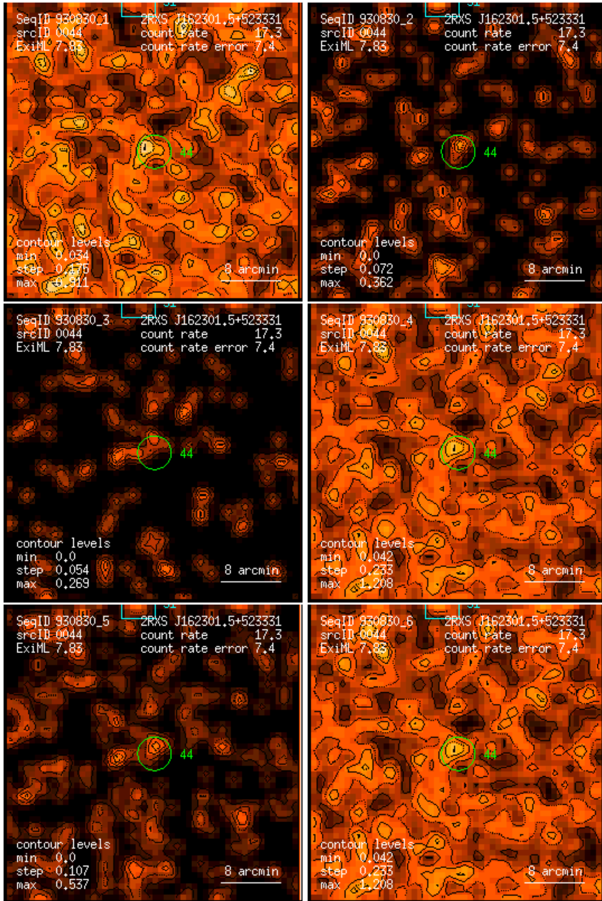
Figure 44: RASS 930830: detection 0044: band rate images, Gaussian filter: (1) PSPC channels 11 – 41, (2) 52 – 90, (3) 91 – 201, (4) 11 – 235, (5) 52 – 201, (6) 11 – 201. Broad band rates in counts/ks. Band rate contour levels in counts/ks/arcmin 2 .
