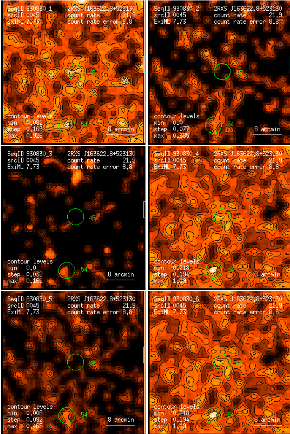
Figure 45: RASS 930830: detection 0045: band rate images, Gaussian filter: (1) PSPC channels 11 – 41, (2) 52 – 90, (3) 91 – 201, (4) 11 – 235, (5) 52 – 201, (6) 11 – 201. Broad band rates in counts/ks. Band rate contour levels in counts/ks/arcmin 2 .
