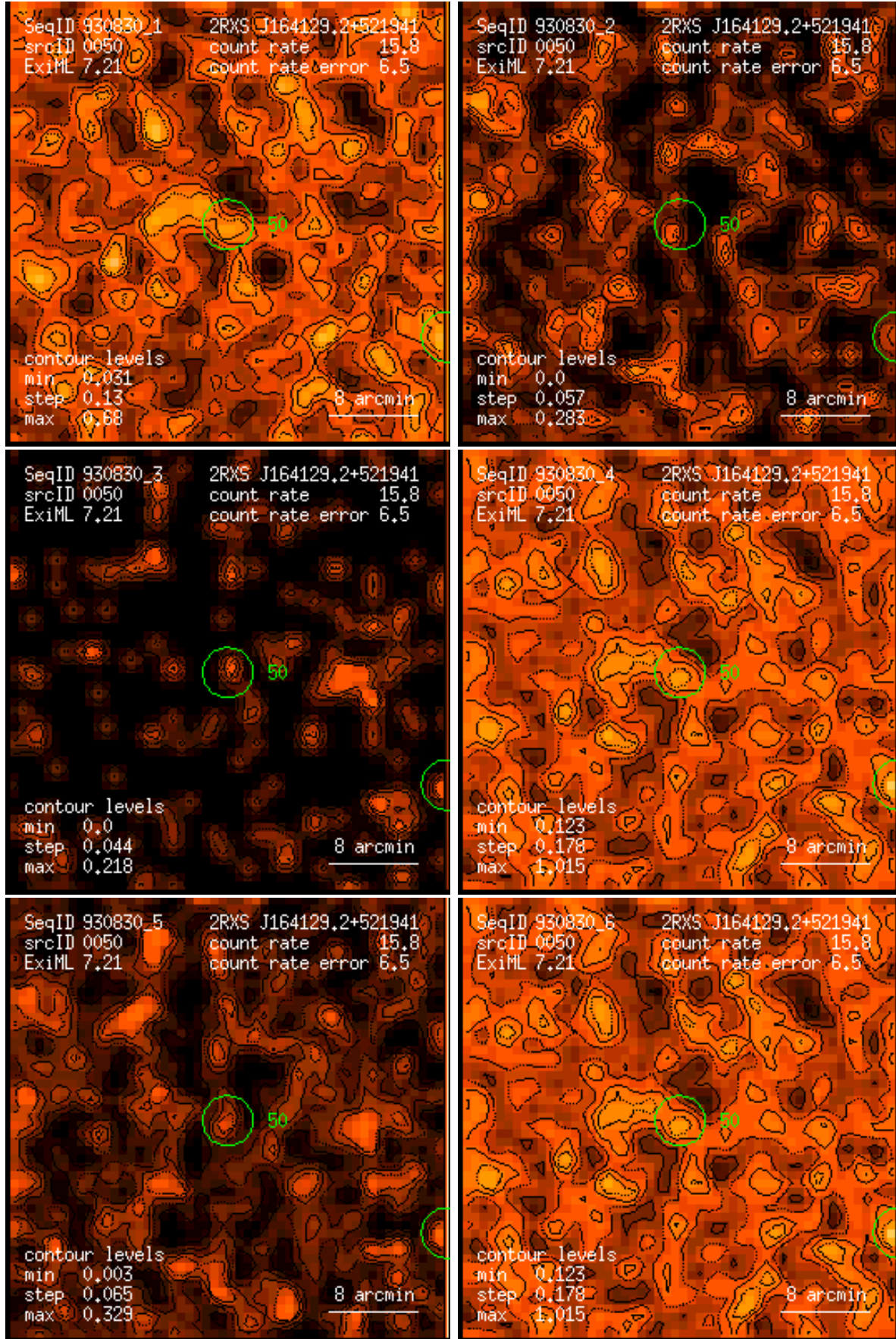
Figure 50: RASS 930830: detection 0050: band rate images, Gaussian filter: (1) PSPC channels 11 – 41, (2) 52 – 90, (3) 91 – 201, (4) 11 – 235, (5) 52 – 201, (6) 11 – 201. Broad band rates in counts/ks. Band rate contour levels in counts/ks/arcmin 2 .
