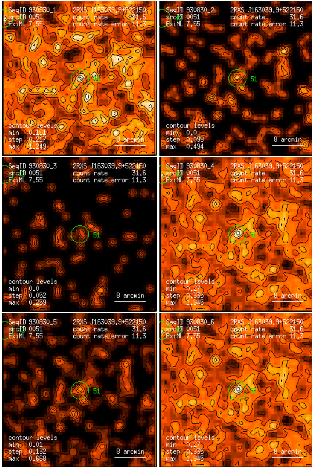
Figure 51: RASS 930830: detection 0051: band rate images, Gaussian filter: (1) PSPC channels 11 – 41, (2) 52 – 90, (3) 91 – 201, (4) 11 – 235, (5) 52 – 201, (6) 11 – 201. Broad band rates in counts/ks. Band rate contour levels in counts/ks/arcmin 2 .
