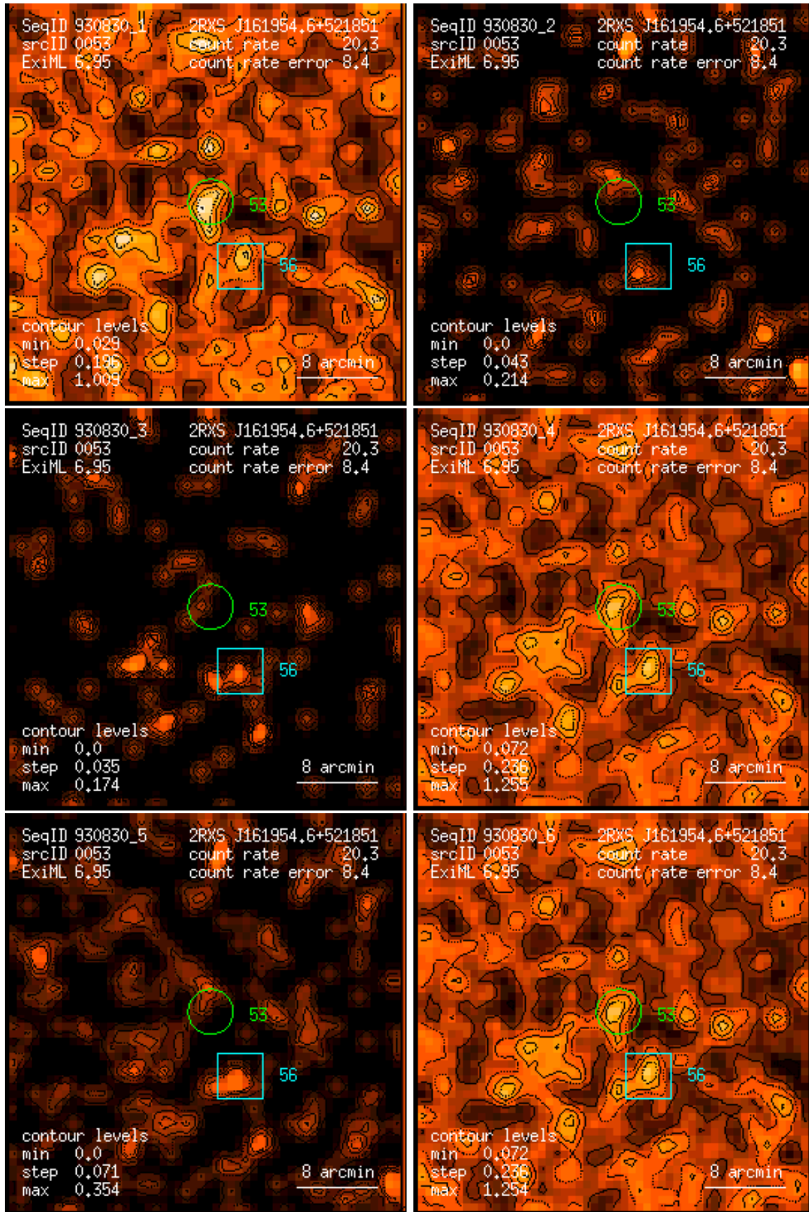
Figure 53: RASS 930830: detection 0053: band rate images, Gaussian filter: (1) PSPC channels 11 – 41, (2) 52 – 90, (3) 91 – 201, (4) 11 – 235, (5) 52 – 201, (6) 11 – 201. Broad band rates in counts/ks. Band rate contour levels in counts/ks/arcmin 2 .
