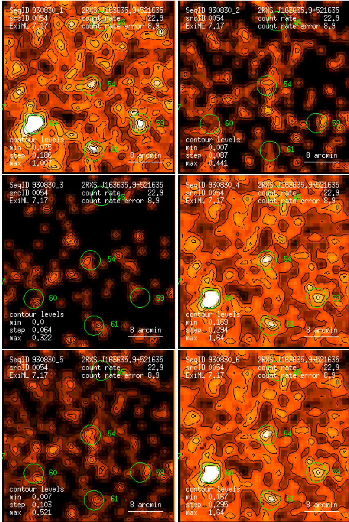
Figure 54: RASS 930830: detection 0054: band rate images, Gaussian filter: (1) PSPC channels 11 – 41, (2) 52 – 90, (3) 91 – 201, (4) 11 – 235, (5) 52 – 201, (6) 11 – 201. Broad band rates in counts/ks. Band rate contour levels in counts/ks/arcmin 2 .
