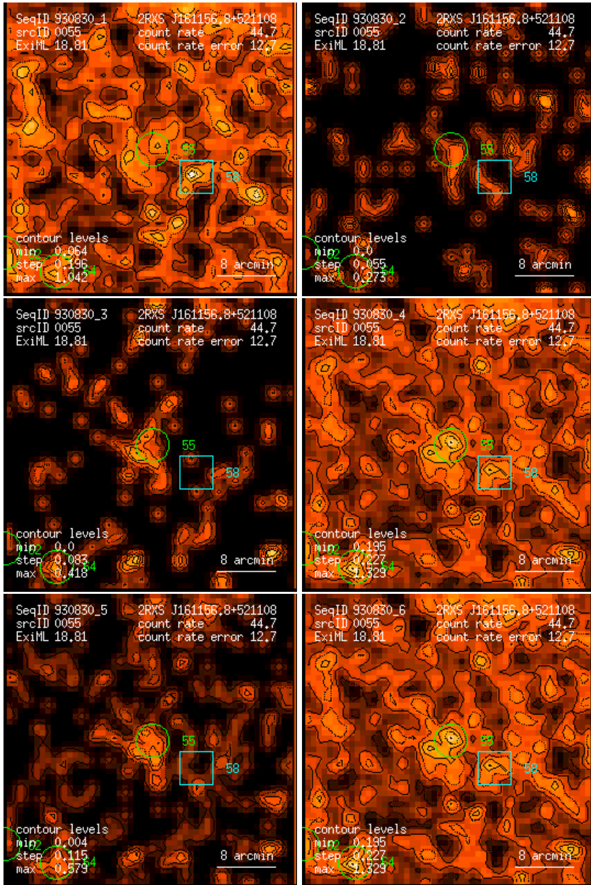
Figure 55: RASS 930830: detection 0055: band rate images, Gaussian filter: (1) PSPC channels 11 – 41, (2) 52 – 90, (3) 91 – 201, (4) 11 – 235, (5) 52 – 201, (6) 11 – 201. Broad band rates in counts/ks. Band rate contour levels in counts/ks/arcmin 2 .
