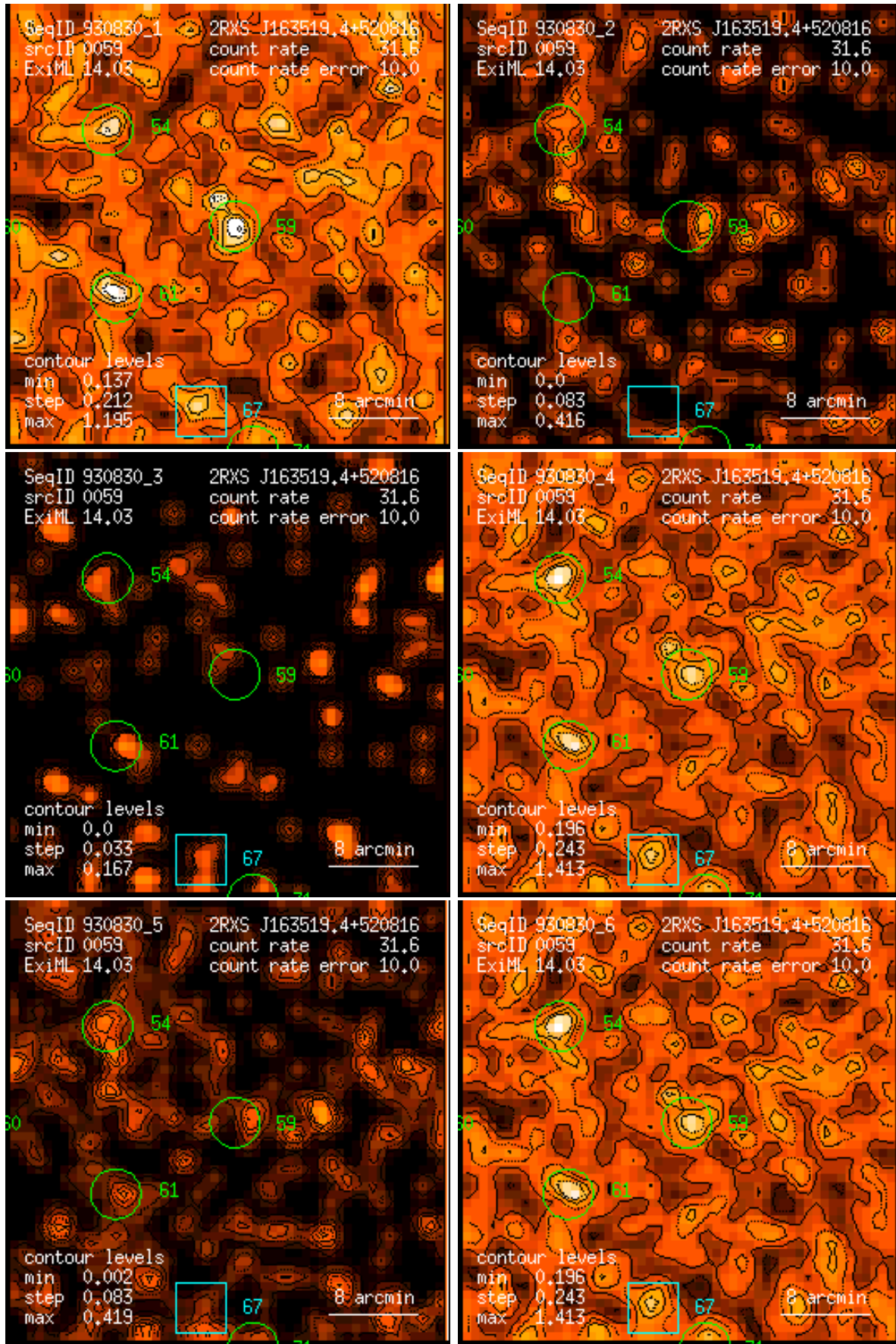
Figure 59: RASS 930830: detection 0059: band rate images, Gaussian filter: (1) PSPC channels 11 – 41, (2) 52 – 90, (3) 91 – 201, (4) 11 – 235, (5) 52 – 201, (6) 11 – 201. Broad band rates in counts/ks. Band rate contour levels in counts/ks/arcmin 2 .
