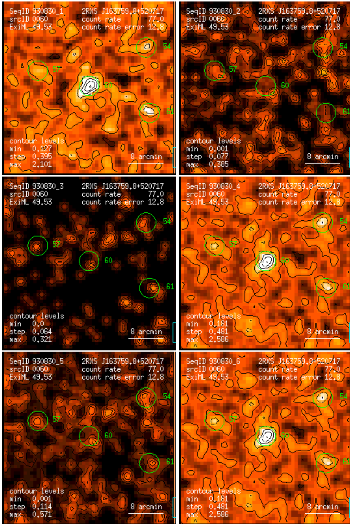
Figure 60: RASS 930830: detection 0060: band rate images, Gaussian filter: (1) PSPC channels 11 – 41, (2) 52 – 90, (3) 91 – 201, (4) 11 – 235, (5) 52 – 201, (6) 11 – 201. Broad band rates in counts/ks. Band rate contour levels in counts/ks/arcmin 2 .
