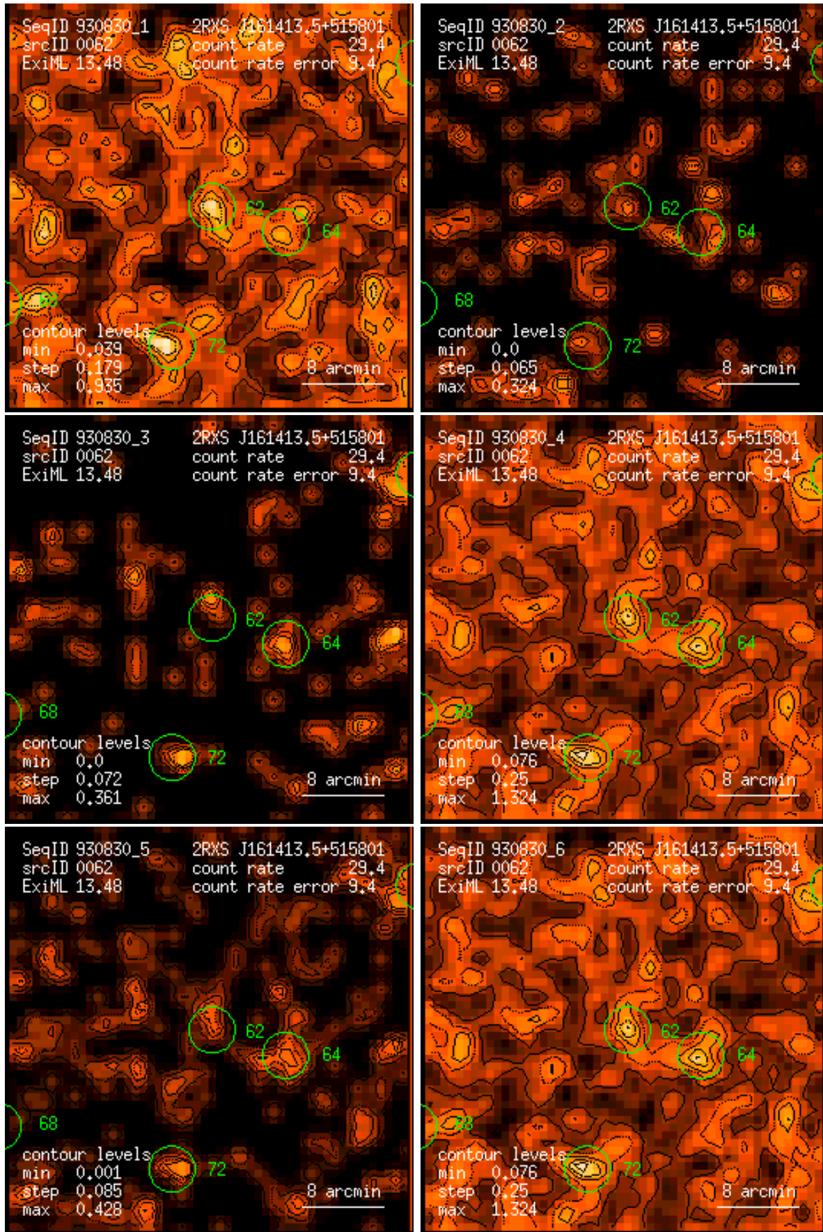
Figure 62: RASS 930830: detection 0062: band rate images, Gaussian filter: (1) PSPC channels 11 – 41, (2) 52 – 90, (3) 91 – 201, (4) 11 – 235, (5) 52 – 201, (6) 11 – 201. Broad band rates in counts/ks. Band rate contour levels in counts/ks/arcmin 2 .
