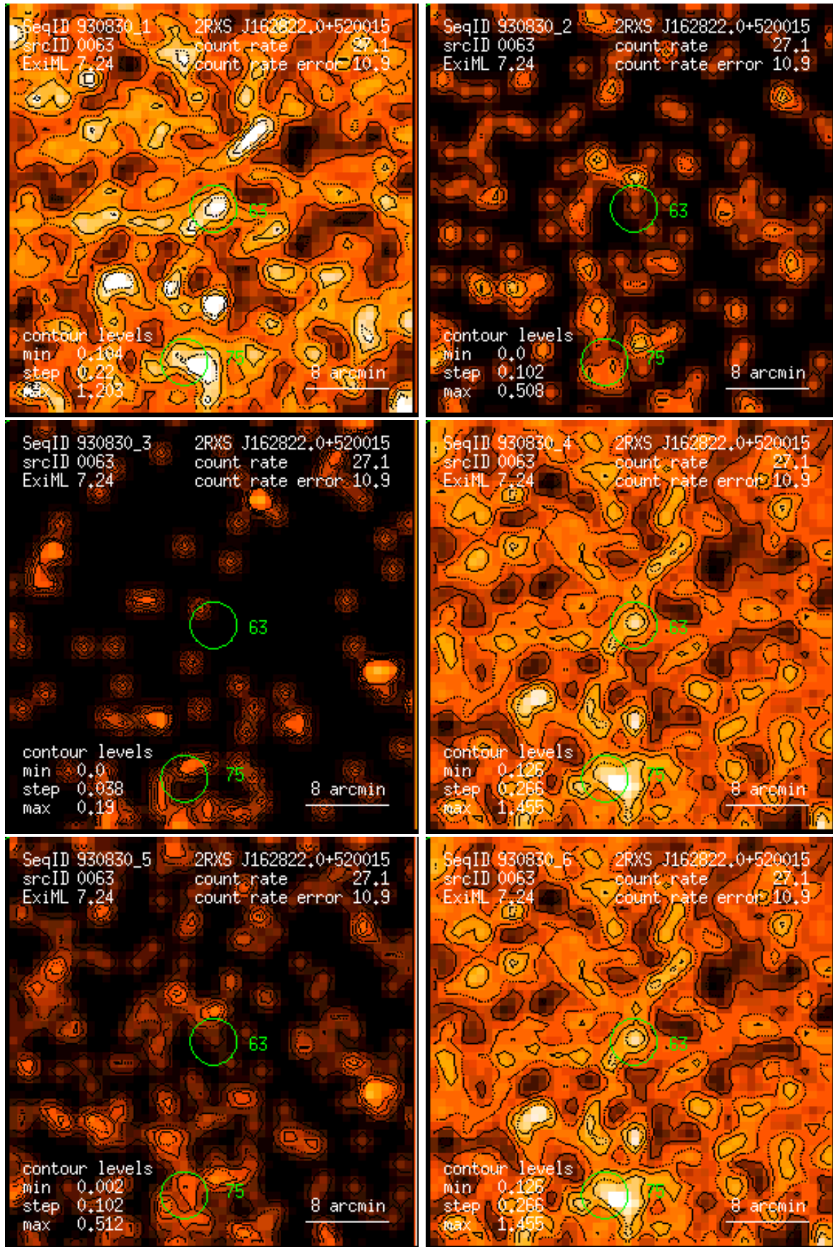
Figure 63: RASS 930830: detection 0063: band rate images, Gaussian filter: (1) PSPC channels 11 – 41, (2) 52 – 90, (3) 91 – 201, (4) 11 – 235, (5) 52 – 201, (6) 11 – 201. Broad band rates in counts/ks. Band rate contour levels in counts/ks/arcmin 2 .
