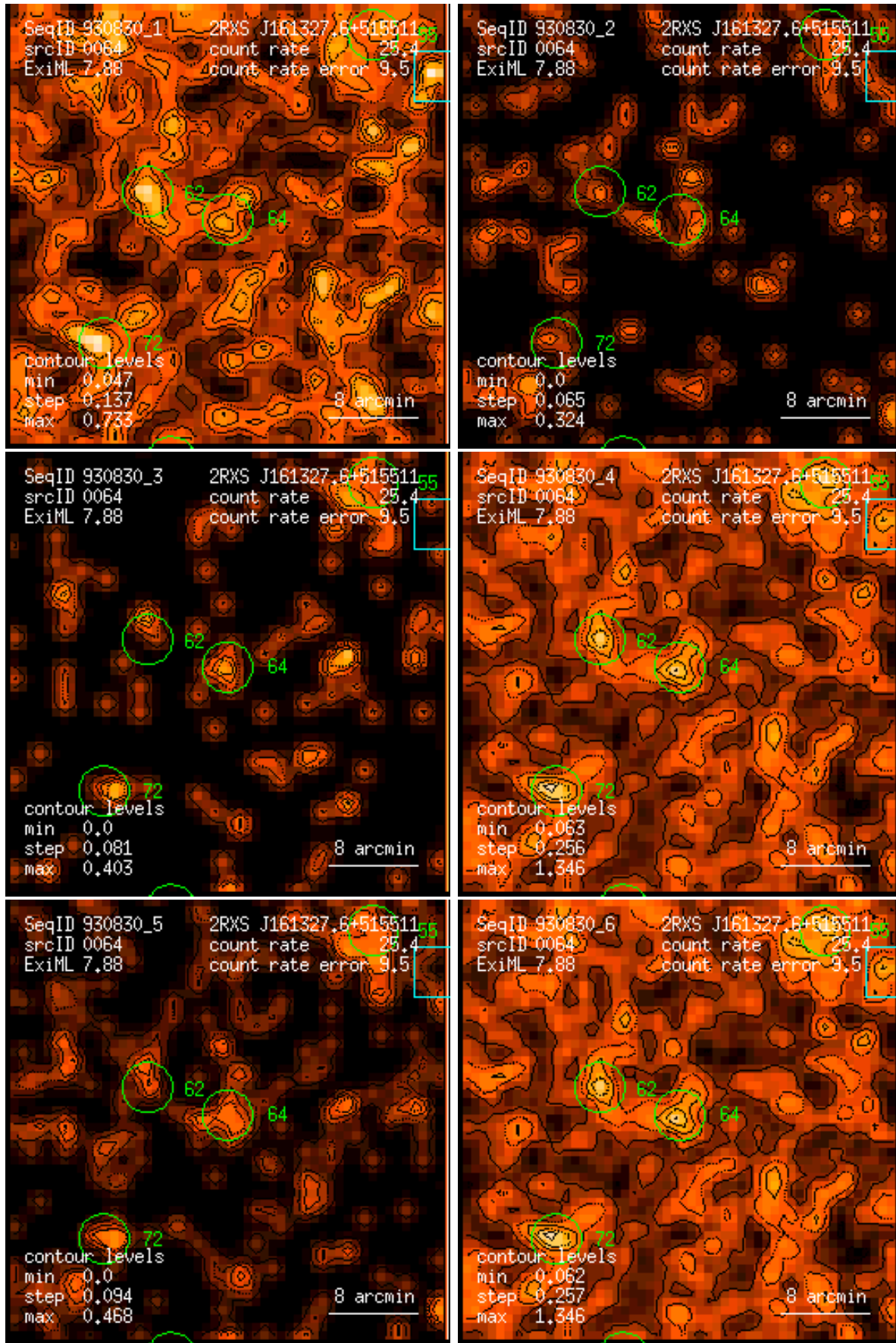
Figure 64: RASS 930830: detection 0064: band rate images, Gaussian filter: (1) PSPC channels 11 – 41, (2) 52 – 90, (3) 91 – 201, (4) 11 – 235, (5) 52 – 201, (6) 11 – 201. Broad band rates in counts/ks. Band rate contour levels in counts/ks/arcmin 2 .
