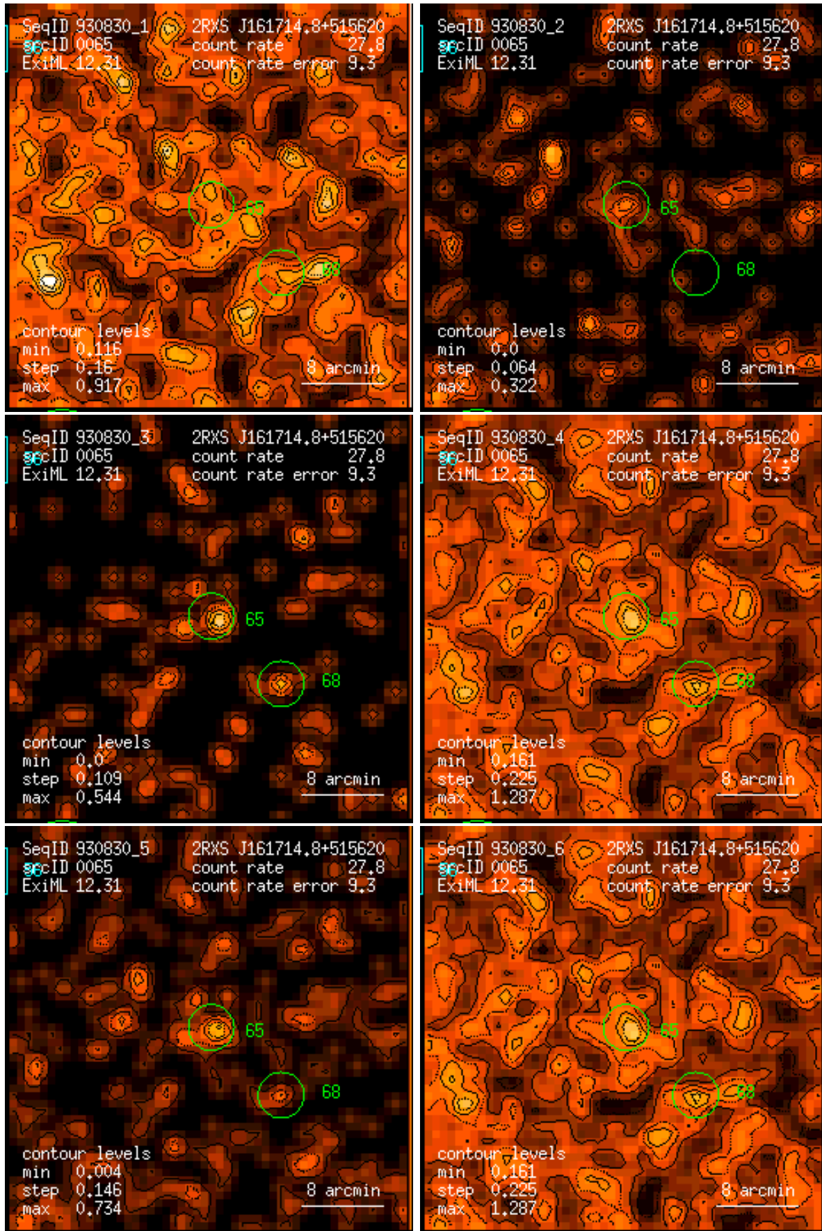
Figure 65: RASS 930830: detection 0065: band rate images, Gaussian filter: (1) PSPC channels 11 – 41, (2) 52 – 90, (3) 91 – 201, (4) 11 – 235, (5) 52 – 201, (6) 11 – 201. Broad band rates in counts/ks. Band rate contour levels in counts/ks/arcmin 2 .
