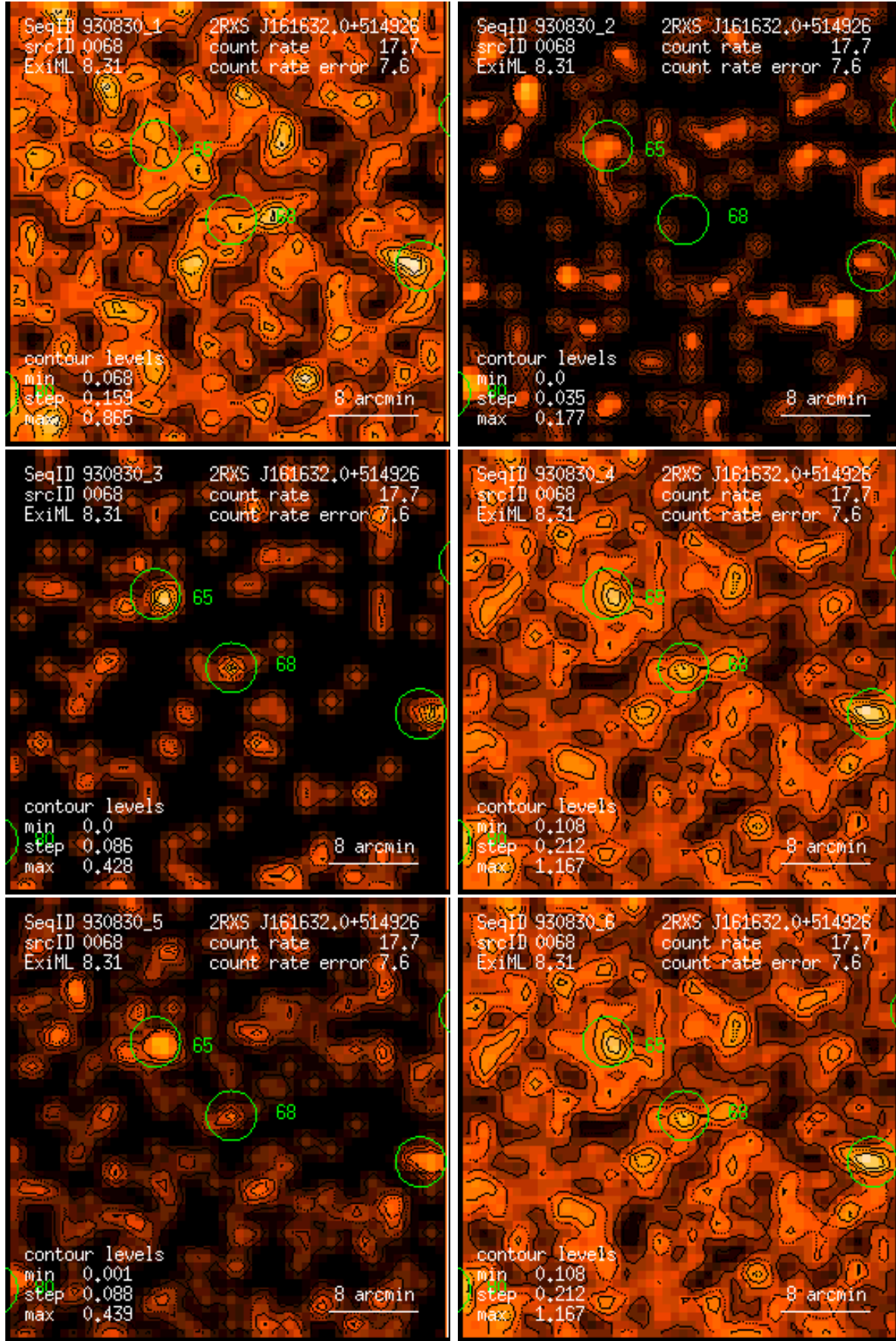
Figure 68: RASS 930830: detection 0068: band rate images, Gaussian filter: (1) PSPC channels 11 – 41, (2) 52 – 90, (3) 91 – 201, (4) 11 – 235, (5) 52 – 201, (6) 11 – 201. Broad band rates in counts/ks. Band rate contour levels in counts/ks/arcmin 2 .
